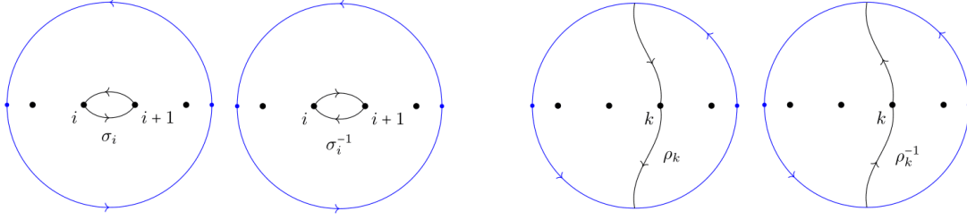
Figure 2.1 The generators \sigma_i and \rho_k , and their inverses, of B_n(\mathbb{R}P^2) .
