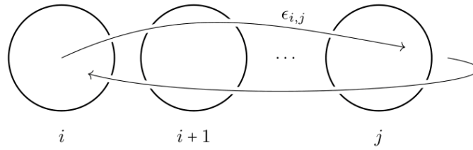
Figure 4.2 The element \epsilon_{i,j} .
