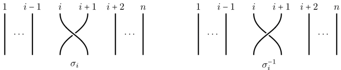
Figure 1.2 The generator \sigma_i and its inverse \sigma_i^{-1} .
