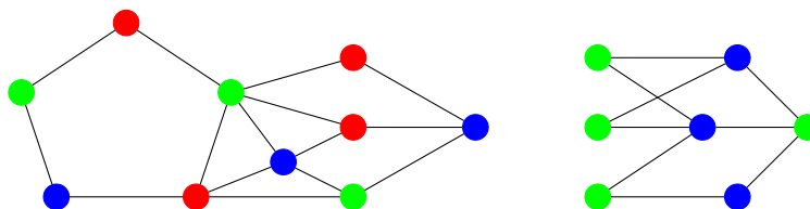
Figure 3.6: Star cutset
