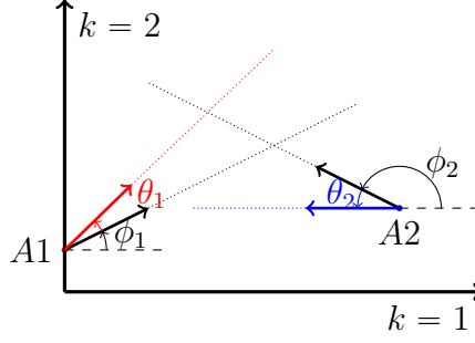
Figure 4.3: Heading angles of two aircraft (in black before deconfliction)
