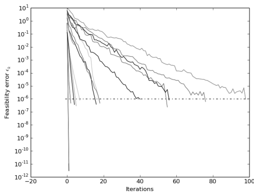
Figure 3.1: Constrained quadratic regression Figure 3.2: Zero-sum game with cubic payoff
