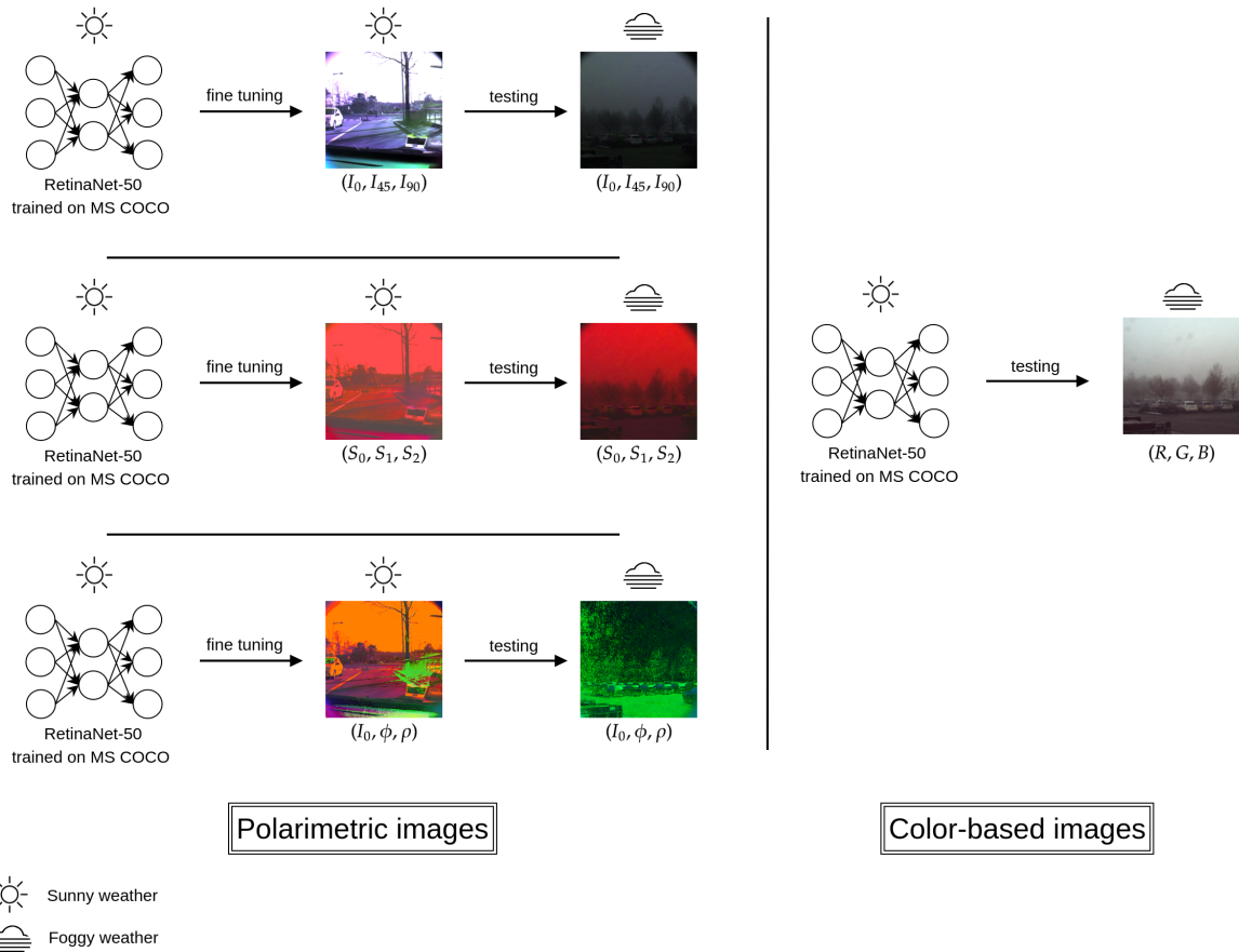
Figure 5.3: Experimental setup. The first column refers to polarimetric data formats, from top to bottom, I , S and pseudo-HSV. Three RetinaNet-50 pre-trained on MS COCO are fine-tuned and tested respectively on I , S and pseudo-HSV. The second column refers to the RGB images. The training set contains scenes in good weather conditions and the testing set contains foggy scenes.
