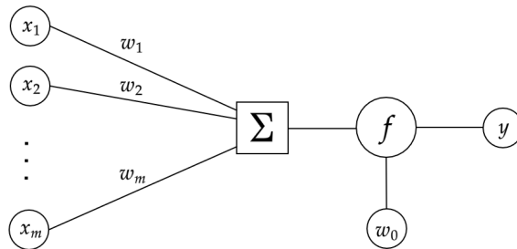
Figure 2.2: Illustration of an artificial neuron. The whole process is summarized up by equation (2.1).
