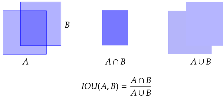
Figure 2.9: Illustration of the Intersection Over Union (IOU) operation. In dark blue, the intersection of bounding boxes A and B and in pale blue the union of bounding boxes A and B .
