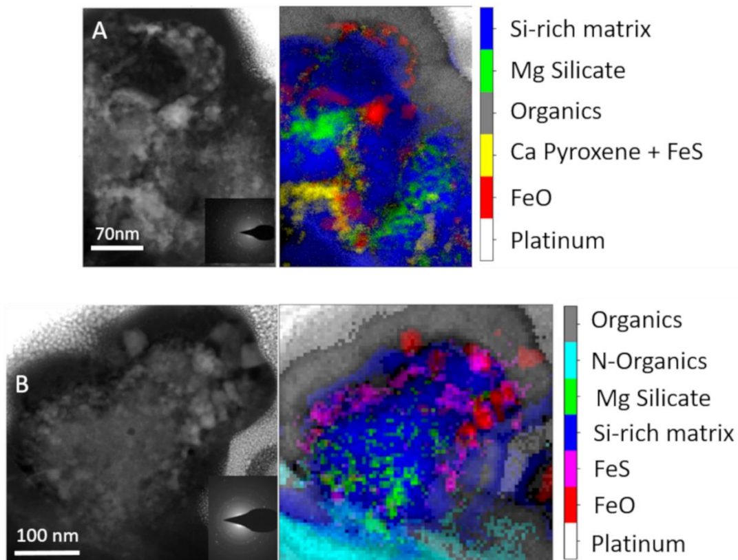
Figure 4-18: (A and B, left) High Angle Annular Dark Field (HAADF) image of 2 mineral assemblages in DC06-308 (A and B, right) False color images corresponding to the EDX maps of the different phases identified by Principal Component Analysis (PCA). The phases are ordered by decreasing number of counts in the respective spectra
