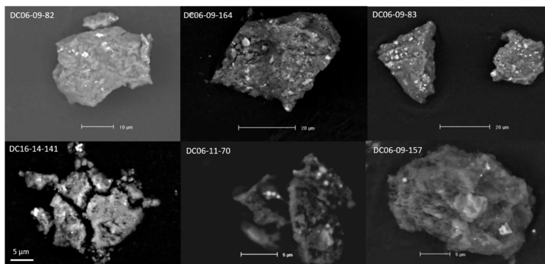
Figure 3-1: Back-scattered Electron (BSE) images of the fragments of 6 hydrated AMMs selected for FTIR analysis.
