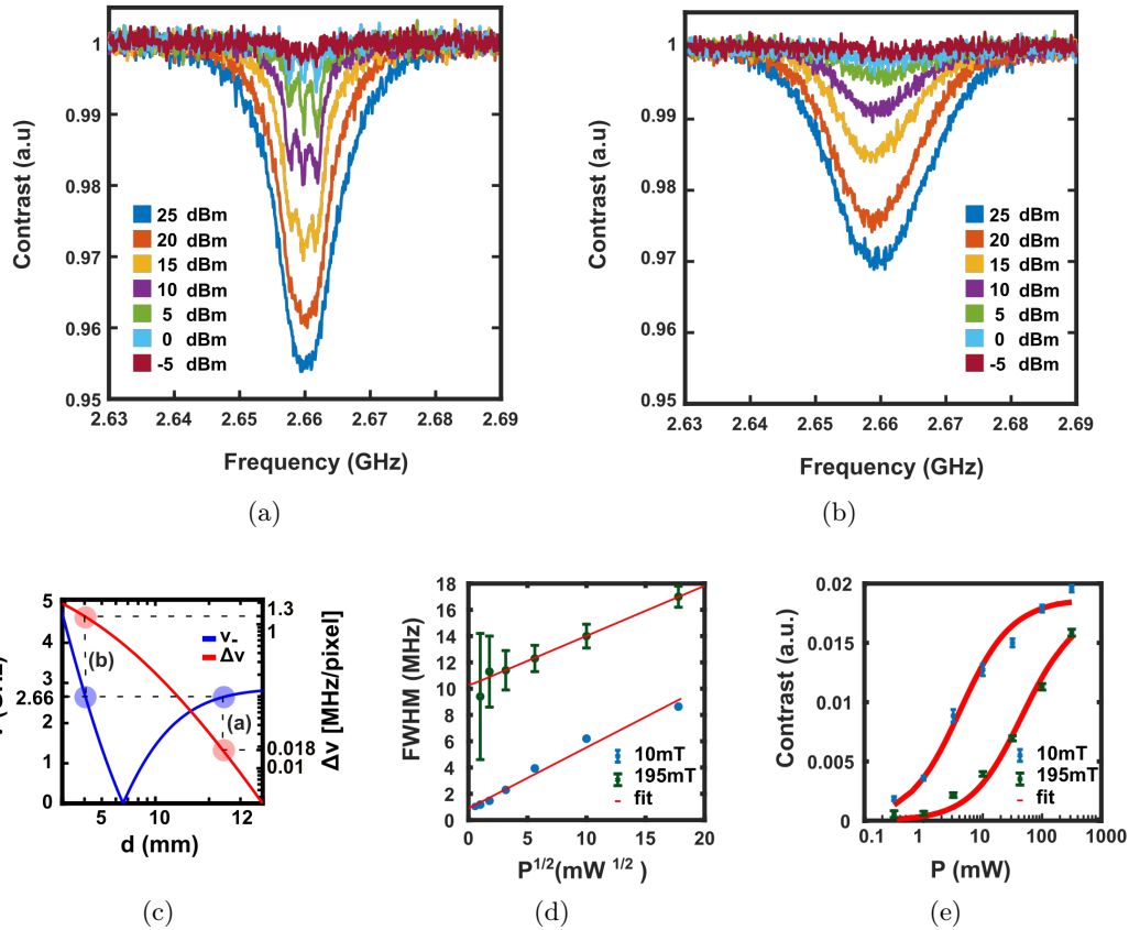
Figure 3.13: Comparison of the ODMR spectra in the range [2.63 GHz, 2.69 GHz] for different magnetic fields and magnetic field gradients (10 mT and 20 KHz/ \mu m (a) – 195 mT and 1.5 MHz/ \mu m (b)). The different colours correspond to different nominal powers of the MW generator. The curves are fitted by the sum of three identical Lorentzians shifted by 2.14 MHz. The contrast and the linewidth obtained from the fit are reported in (c – d). In (c) the fit is realized using a fit function of the form of eq. (3.5); in (d) the fit is realized using a fit function of the form of eq. (3.11) for (d).
