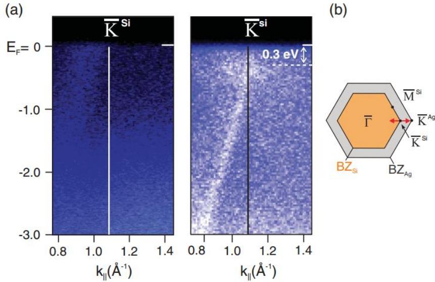
Figure 2.8 (a) ARPES maps for the bare Ag(111) (left) and silicene/Ag(111) (right), along the \bar{\Gamma}_{Ag} - \bar{K}_{Ag} . (b) Brillouin-zone (BZ) scheme for the unit cell of Ag(111) and silicene. The direction of measurements is indicated by the red arrow. Figures reproduced from ref. [5]
