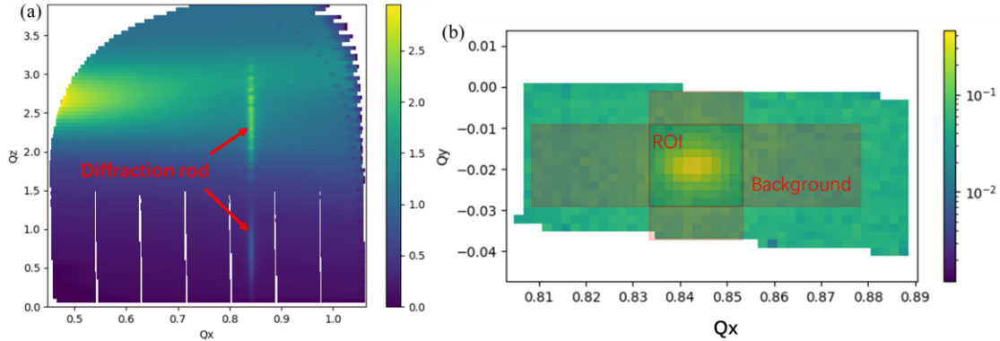
Figure 3.14 (a) Diffraction rod related to the (3 \times 3) reconstruction of Ge on Al(111). (b) The selected ROI and the background in a slice of a diffraction rod for the fitting and integration by BINoculars.
