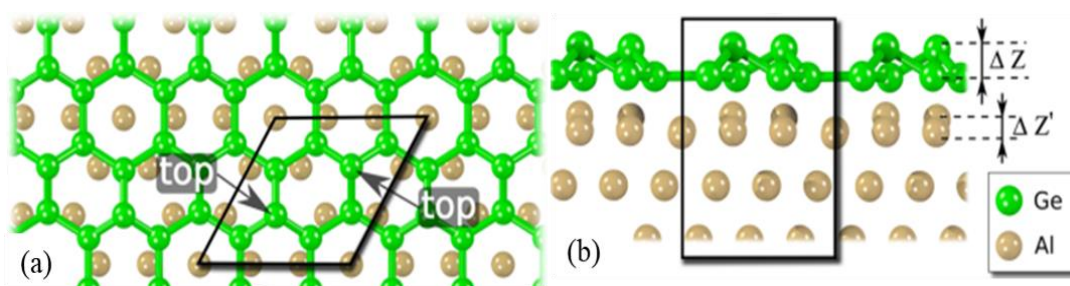
Figure 2.14 Top (a) and lateral (b) view of the atomic model of germanene grown on Al(111). The black rhombus shows the unit cell of germanene with two protruding Ge atoms labeled “top”. The black rectangle is the lateral view of the rhombus zone in (a). Image reproduced from ref. [7]
