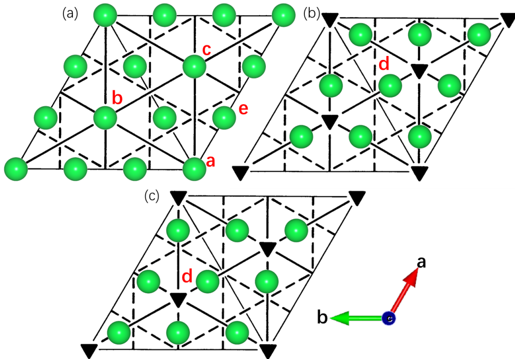
Figure 4.14 Atomic configuration for Al(111) planes with the p3m1 symmetries. Different configurations are indicated by Wyckoff position (a) abce and (b), (c) ddd , respectively. Mirror and glide planes are drawn in black continuous and dotted lines respectively. Triangles indicates 3-fold rotation axes. Lattice vectors are indicated by the red and green arrow.
