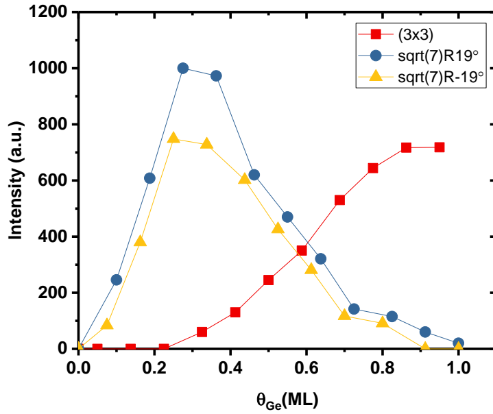
Figure 4.13 Evolution of the diffracted intensity for the (2/3, 0, 0.1) (red squares), (4/7, 1/7, 0.1) (blue circles) and (5/7, -1/7, 0.1) (yellow triangles) position related to the (3 \times 3) and (\sqrt{7} \times \sqrt{7}) reconstruction, during Ge deposition on the Al(111) surface kept at 333K.
