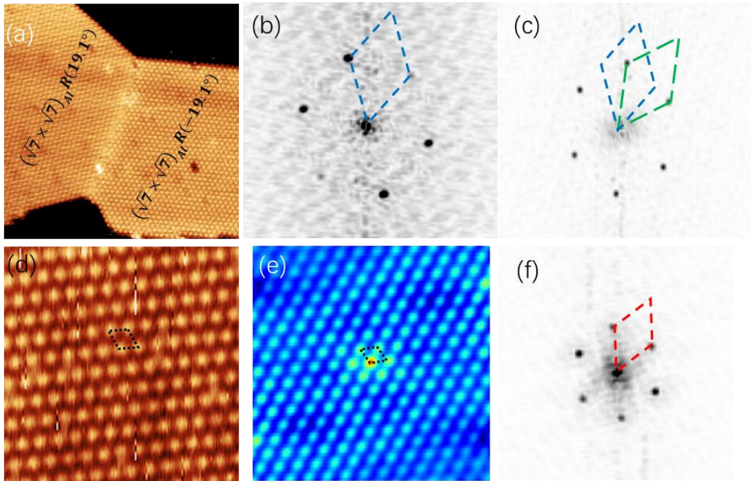
Figure 4.3 (a) Atomic resolution STM image of the (\sqrt{7} \times \sqrt{7}) ( 40 \times 40 \text{ nm}^2 ; U=2.0\text{V} , I=30 \text{ pA} ). The left part corresponds to the (\sqrt{7} \times \sqrt{7})R19.1^\circ reconstruction, while the right part indicates the (\sqrt{7} \times \sqrt{7})R-19.1^\circ one. (b, c) Corresponding Fast Fourier Transform images related to the left and right part of (a). The dashed blue and green rhombus denote the hexagonal unit cell of the (\sqrt{7} \times \sqrt{7})R \pm 19.1^\circ in the reciprocal space. (d) Atomic resolution STM image of the (3 \times 3) reconstruction ( 10 \times 10 \text{ nm}^2 ; U=0.9\text{V} , I=50 \text{ pA} ). The unit cell of the (3 \times 3) reconstruction is indicated by the dotted black rhombus. (e) Corresponding self-correlation images. The dotted black rhombus represents the unit cell of the (3 \times 3) reconstruction. (f) Corresponding Fast FFT images.
