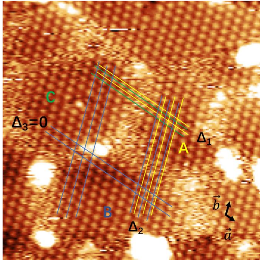
Figure 4.4 Detailed view of the (\sqrt{7} \times \sqrt{7}) reconstruction. The yellow, blue, and green solid lines indicate the direction of the atomic rows in three areas labeled as A, B, and C with different colors, respectively. \Delta is the shift of the atomic rows. The vector \vec{a} and \vec{b} represent the lattice vectors of the (\sqrt{7} \times \sqrt{7}) unit cell. Size of the images 20 \times 20 \text{ nm}^2 . Tunneling conditions: V_S = 0.9 \text{ V} , I = 50 \text{ pA} .
