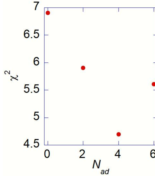
Figure 6.9 Evolution of the value of \chi^2 for the (13×4) phase as a function of the number of Si adatoms in the unit cell ( N_{ad} ).
