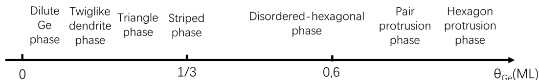
Figure 5.1 Evolution of the formation of the different phase depending on Ge coverage. The completion of the striped phase corresponds to 1/3ML as a reference.
