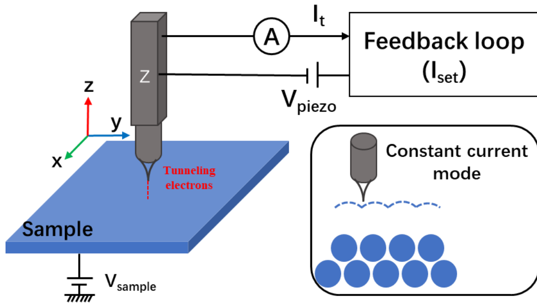
Figure 3.1 Schematic representation of the effect of the feedback loop. For each point the voltage used to the z-piezodrive to adjust the tip at the distance for the constant tunneling current I_{\text{set}} ; I_t and I_{\text{set}} are respectively the tunneling current and the current requested by the user. Inset: Schematic of the constant current acquisition mode.
