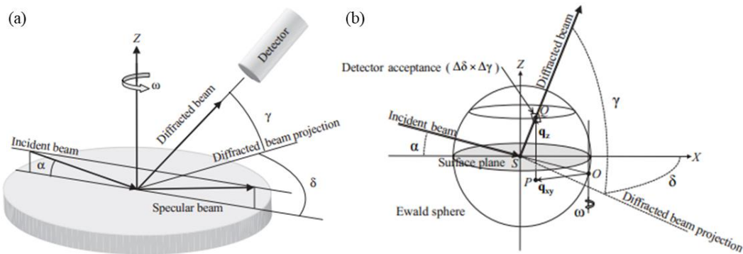
Figure 3.13 (a) Schematic diagram of the Z-axis diffractometer geometry exhibiting the incident angle \alpha , the sample rotation around Z-axis by \omega , and the azimuths \gamma and \delta . (b) Perspective view of Ewald sphere. Images reproduced from ref. [124]
