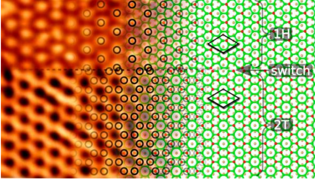
Fig 2.16 Experimental STM image ( U = 1\text{ V} ) and the network of two simulated structures, showing the switching between 1H and 2T configuration. The unit cell (black rhombus) of the 1H configuration shows only one protruding Ge atom (red ball), instead of two in the 2T configuration. Green and beige balls correspond to Ge and Al atoms, respectively. The black circles show the correspondence between the uplifted Ge atoms in the calculated network and the protrusions in the STM image. Figure adapted from ref. [96]
