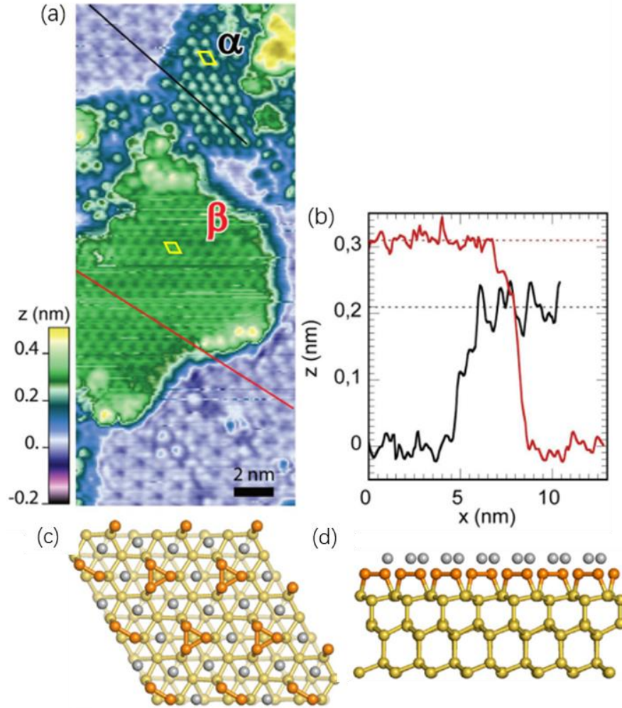
Figure 2.10 (a) STM image ( 11 \times 25 \text{ nm}^2 ; U=1.6 \text{ V} , I=50 \text{ pA} ) after Si deposition at 500K above 1 ML. Two types of the (\sqrt{3} \times \sqrt{3})R30^\circ reconstruction show a different contrast, the unit cell of them is presented by the yellow rhombus. (b) Profiles along the lines shown in (a). (c) Top and (d) side views of the HCT model applied for fitting the experimental structure factors measured by GIXD. The small grey balls represent Ag atoms. The yellow balls represent Si atoms, while the protrusive Si atoms are drawn in orange. Figure reproduced from ref. [34], [35]
