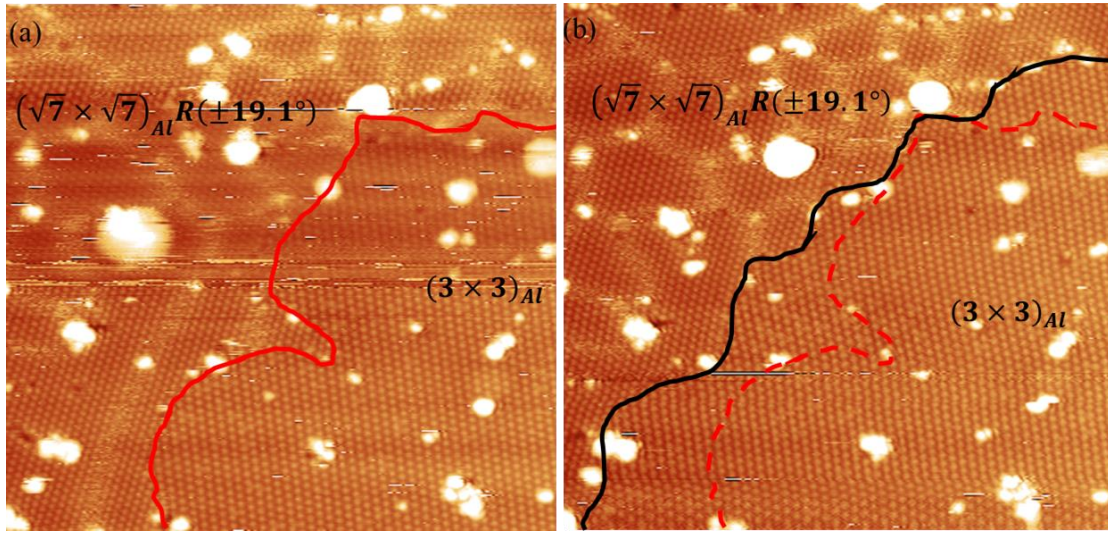
Figure 4.7 Evolution of the (3 \times 3) and (\sqrt{7} \times \sqrt{7}) reconstruction domains during Ge deposition on Al(111) held at 357K shown in two adjacent STM images with a time interval of 10 min. In (a), the boundary between the (3 \times 3) and (\sqrt{7} \times \sqrt{7}) areas is marked by a red solid line. In (b), the previous and new boundaries are indicated by a red dotted and black solid lines. Size of the images 48 \times 47 \text{ nm}^2 . Tunneling conditions: V_s = 0.9 \text{ V} , I = 50 \text{ pA} .
