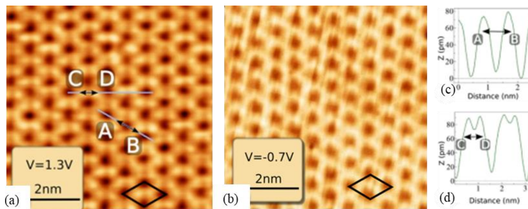
Figure 2.13 High-resolution STM image (a) in positive bias ( U = 1.3 V, I = 0.3 nA) and (b) in negative bias ( U = -0.7 V, I = 0.3 nA) of germanene/Al(111). The black rhombus shows the unit cell of germanene. The line profiles along AB and CD in (a) are drawn in (c) and (d), respectively. Image reproduced from ref. [7]
