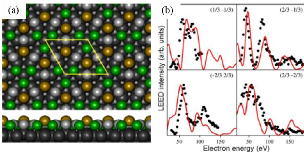
Figure 2.19 (a) Top and lateral view of the relaxed model of Ge-Al alloy. Yellow and green balls indicate Ge atoms in a higher and lower position, respectively. Gray and black balls represent Al atoms in the top layer and in the underlying layer, respectively. (b) Comparison between experimental (black dot) and simulated LEED I-V curve (red line, corresponding 4 spot: (1/3 -1/3) , (2/3 -1/3) , (-2/3 2/3) , and (2/3 -2/3) ). Figures reproduced from ref. [93]
