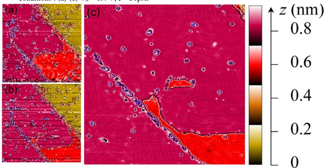
Figure 5.12 Evolution of the Ag(111) surface during Ge deposition at 380K. (a) and (b):consecutive images ( 170 \times 170 \text{ nm}^2 ) acquired at 40 min time interval showing the motion of the outgrowth edge. The detail (c) show that the outgrowth is uniformly covered with the striped phase, as in the initial terrace. Tunneling conditions : V_s = 1.5 \text{ V} ; I = 30 \text{ pA} .
