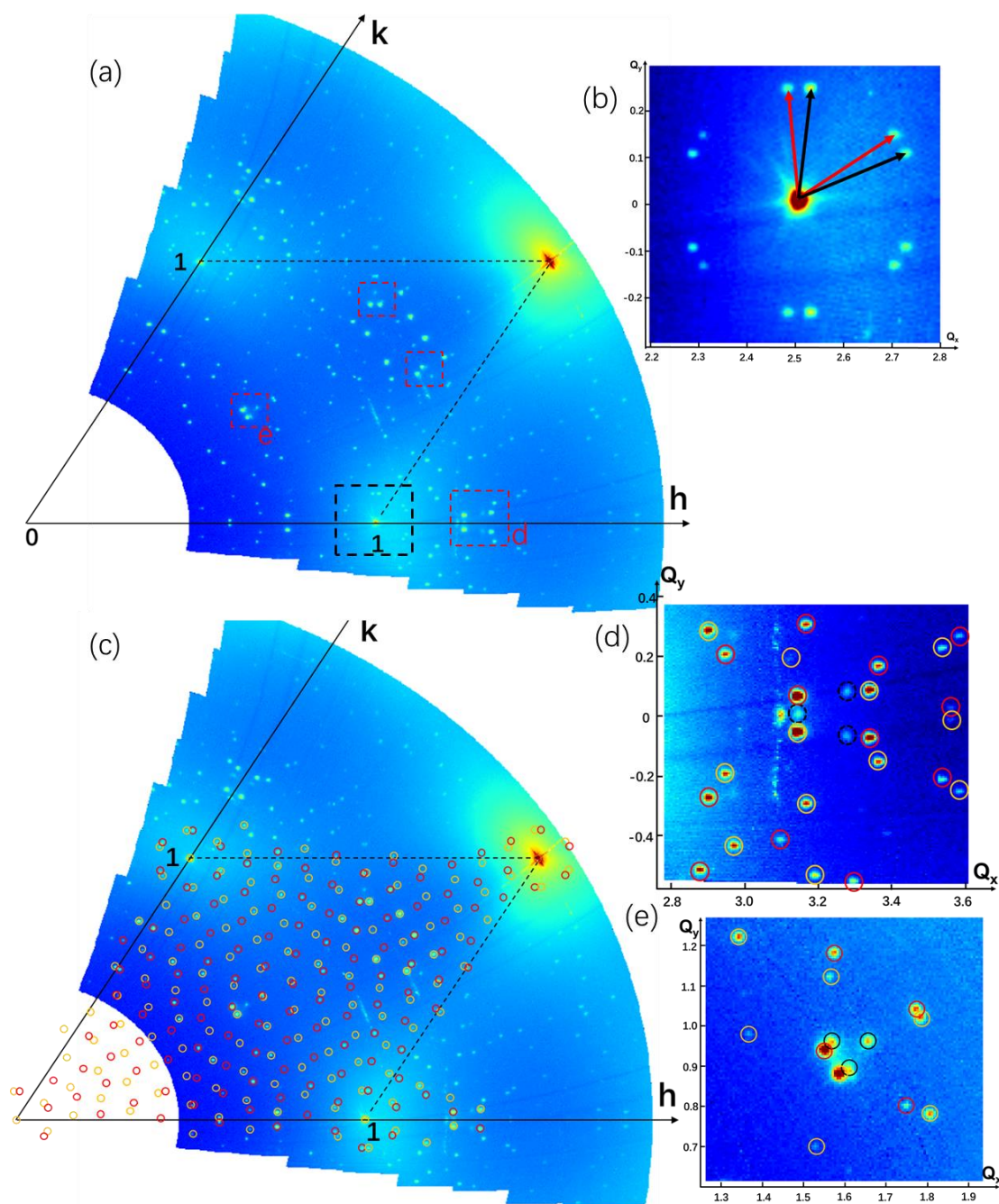
Figure 5.20 Diffracted intensity for in-plane conditions ( l=0.12 ) after evaporation of \theta_{Ge} \approx 1 ML. (a) large view of the reciprocal space. The black dashed parallelogram corresponds to the Ag(111) surface unit cell. (b) A detailed view around (h=1, k=0) condition, as indicated by the dotted black square shown in (a). (c) Schematic representation of the diffraction spots and rods for the (\sqrt{109} \times \sqrt{109})_{Ag} R \pm 5.5^\circ reconstruction. Red and yellow circles indicate the (h, k, 0.12) positions associated with the (\sqrt{109} \times \sqrt{109})_{Ag} R \pm 5.5^\circ reconstruction in the reciprocal space. (d)-(e) detailed view around (h=9/7, k=0) and (h=3/7, k=3/7) condition, as indicated by the dashed red square shown in (a). The black (dashed) circles indicate the diffraction spots uncorrelated with the (\sqrt{109} \times \sqrt{109})_{Ag} R \pm 5.5^\circ reconstruction and minor intensity.
