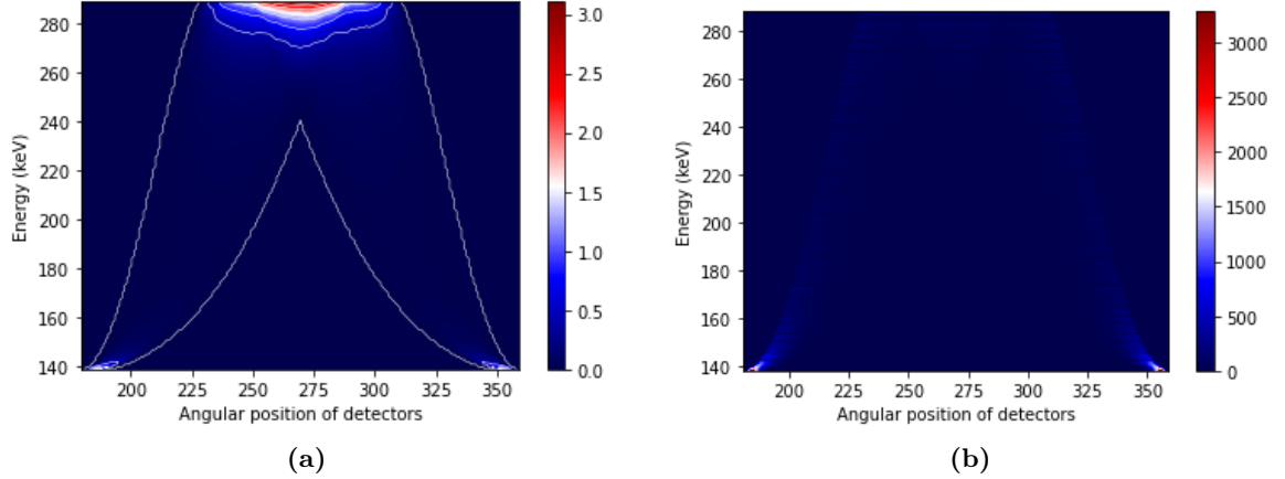
Figure A.3 – (a) Acquisition data obtained from the expression of the generalized Radon transform (3.9). Comparison with (b) acquisition data by Monte Carlo simulations.
