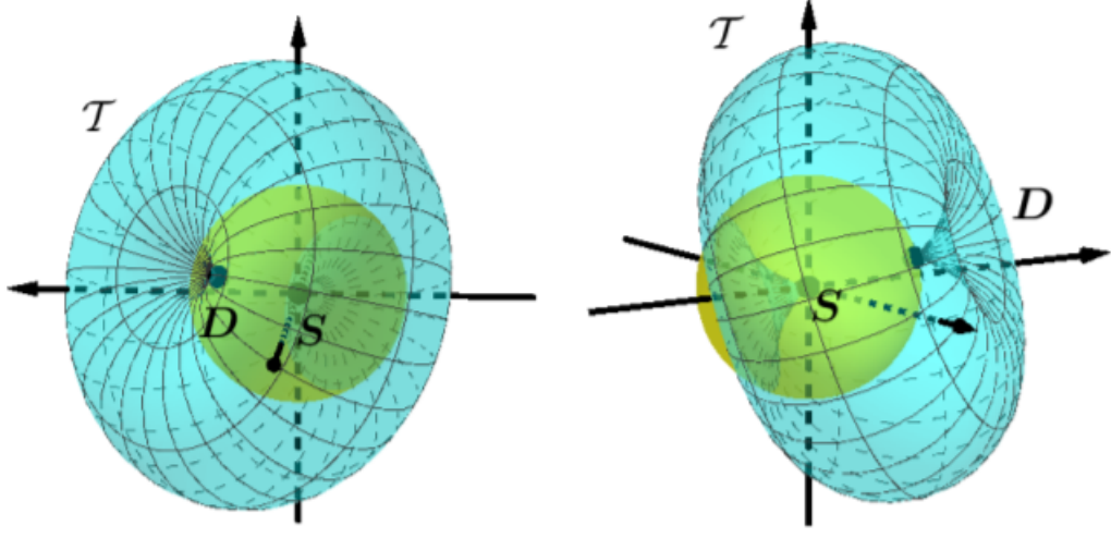
Figure 7.7 – Two views of the three-dimensional fixed source rotating detector CST modality. The detector D moves on a sphere in yellow. A particular scattering toric surface \mathcal{T} is showed in blue.
