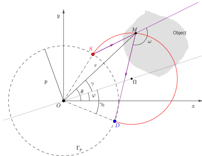
Figure 1.9 – Truong and Nguyen’s modality - 2011. The colour code is the same as in figure 1.7. The dashed circle represents the circular path on which moves the pair source-detector.
