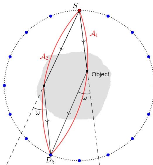
Figure 3.1 – Presentation of CCST. The dotted line represents the ring containing point-like detectors in blue. We find also the source, in red, on the ring. For an arbitrary detector D_k and a scattering angle \omega , the corresponding double scanning arc \mathcal{A}_1 \cup \mathcal{A}_2 is showed in red.
