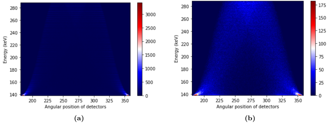
Figure A.4 – Validation of the proposed model with Monte Carlo simulation results for (a) all combined scattering orders and (b) second scattering order only.
