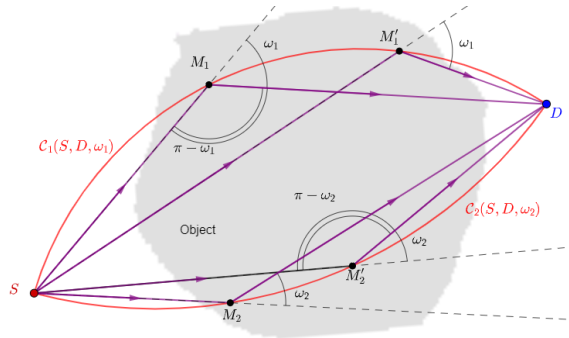
Figure 1.6 – General functioning principle of a CST system. Photons are emitted by source S (in red), interact at sites M , and are recorded at site D (in blue). When a photon is detected carrying an energy E(\omega_1) (resp. E(\omega_2) ), the possible interaction sites lie on the upper (resp. lower) circle arc which subtends the angle (\pi - \omega_1) (resp. (\pi - \omega_2) ).
