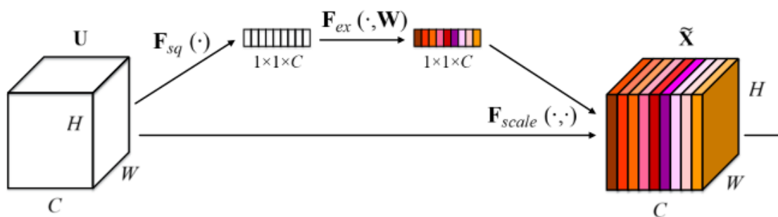
Figure 2.7 – Squeeze-and-Excitation computation. The input feature maps are first squeezed per channel through global average pooling. The excitation block learns from the channel descriptors the scale that is then applied to the input features maps to emphasize relevant channels. Source [Hu et al., 2018], modified.
