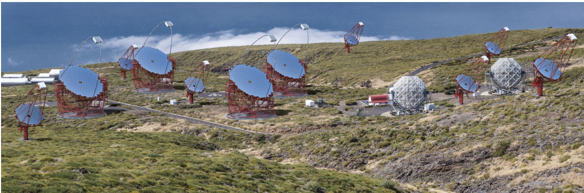
Figure 1.15 – CTA, La Palma site. Credit: Gabriel Pérez Diaz, IAC
