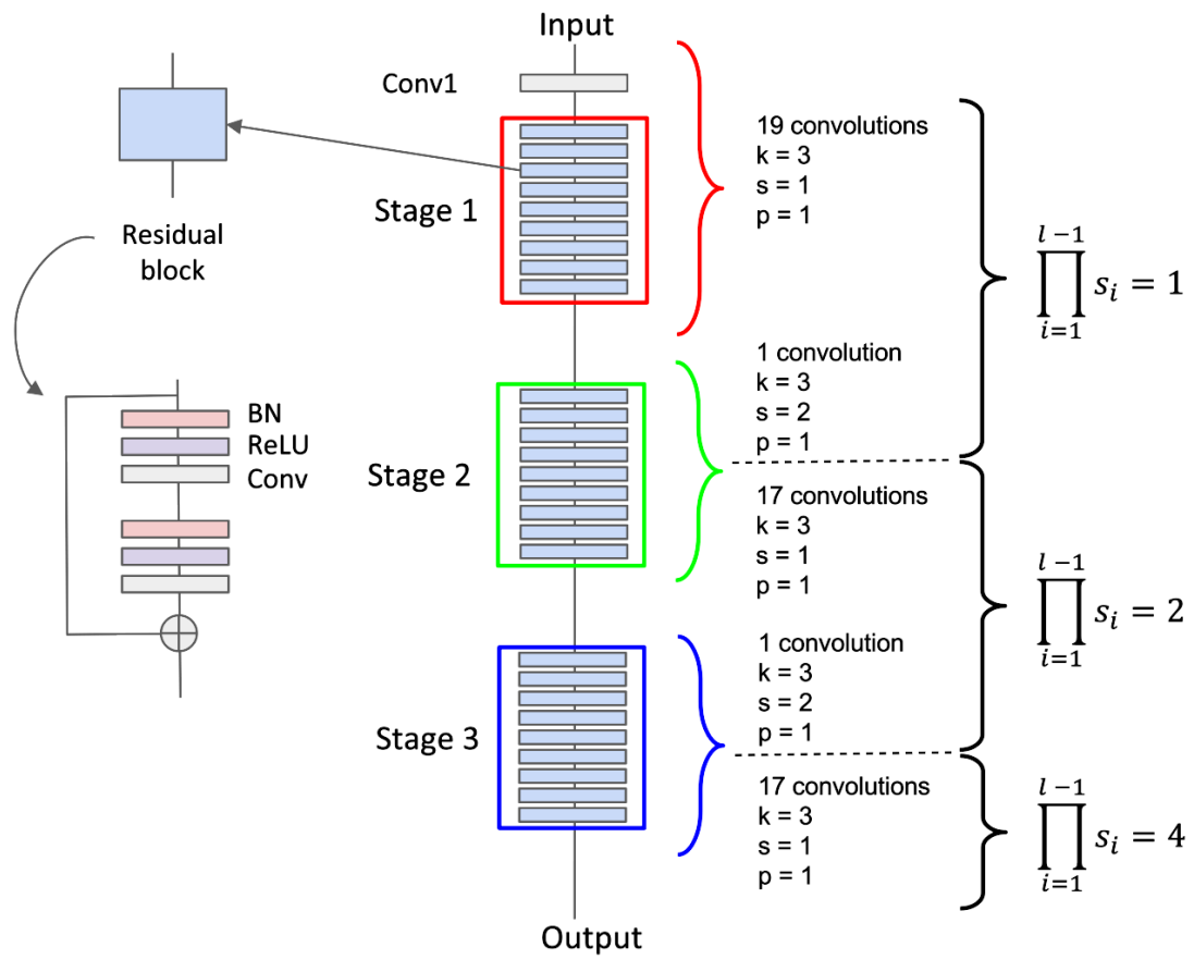
Figure E.1 – \gamma -PhysNet Receptive Field Computation.
