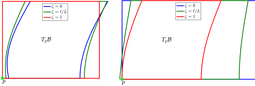
FIGURE 5.11: Developing curve \tilde{\sigma} obtained for various \zeta and for the transformations (5.5.22) (left) and (5.5.26) (right).
