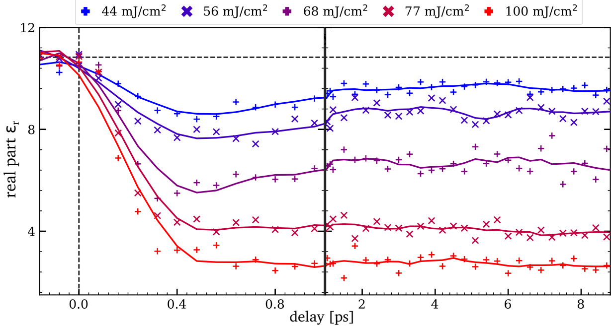
Figure 5.14 – Real part of the dielectric function as a function of delay for the GSSN sample. The horizontal dotted line highlights the value in the initial state \epsilon^{cold}(532 \text{ nm}) = 10.83 + 4.36 i . Solid lines are guides to the eyes.
