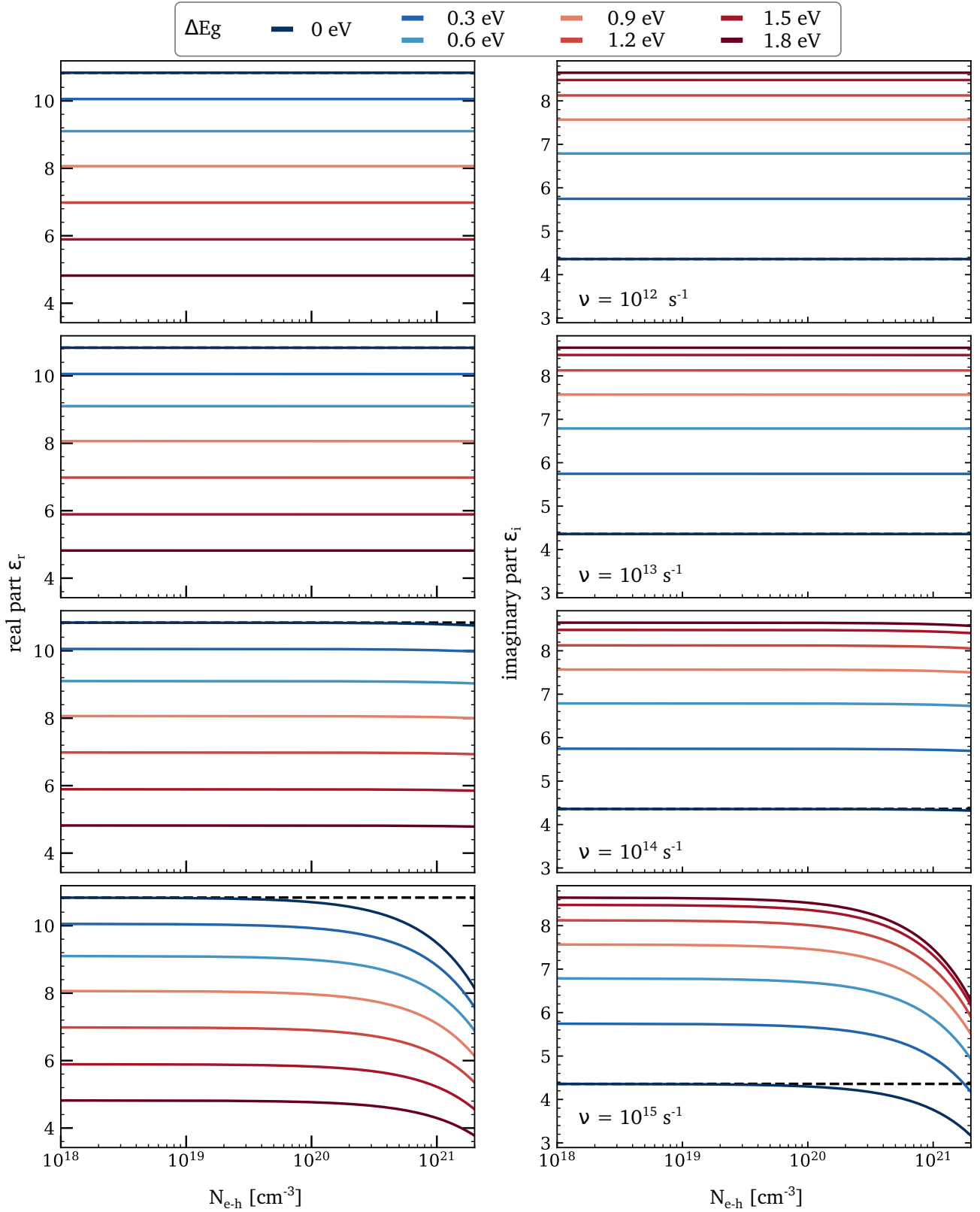
Figure D.4 – Excited dielectric function at 532 nm for GSSN. The horizontal dotted line shows the value of \epsilon^{\text{cold}}(532 \text{ nm}) = 10.83 + 4.36i .
