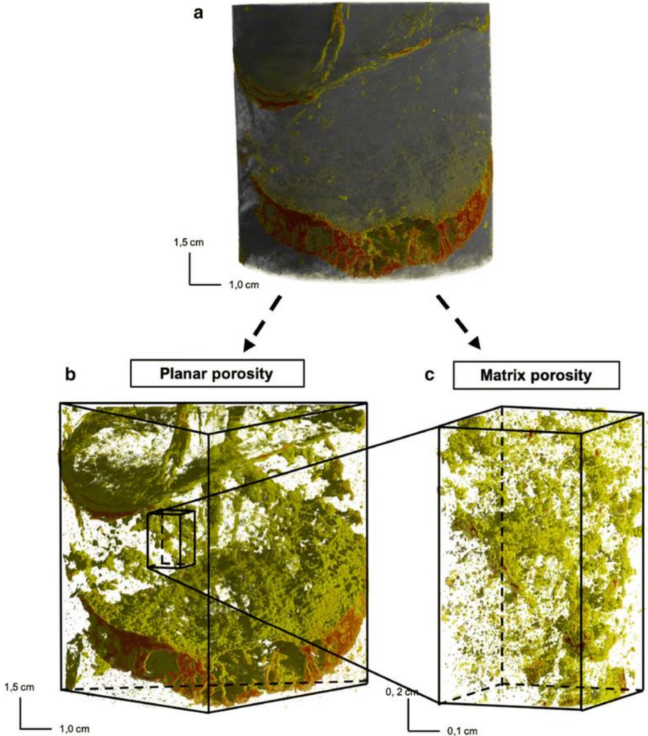
Figure 58 : Three-dimensional observations of the planar and matrix porosity of one sample taken from the Pont-gibaud fault zone. The red color of figures (a), (b), corresponds to mineralization (lead sulphides). The yellow color of figures (a), (b) corresponds to the planar porosity located on the fracture walls. The yellow color of figure (c) could correspond to the matrix porosity. The resolution of figures (a)-(c) is, respectively, 25, 25 and 4 \mu\text{m} .
