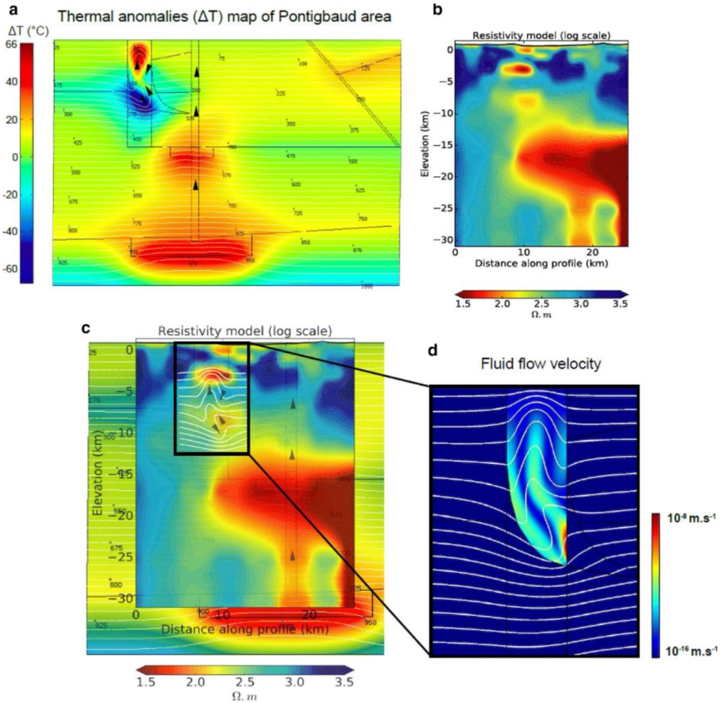
Figure 64 : (a) Thermal anomalies maps of Pontgibaud area. The black arrows represent the direction of fluid flow. (b) Resistivity model previously described (Fig 43). (c) Comparison of the numerical simulation result affecting a K_{max} permeability of 1.6 \times 10^{-14} \text{ m}^2 at the Pontgibaud fault zone, with the resistivity profile. (d) Fluid flow velocity within the Pontgibaud Crustal fault Zone.
