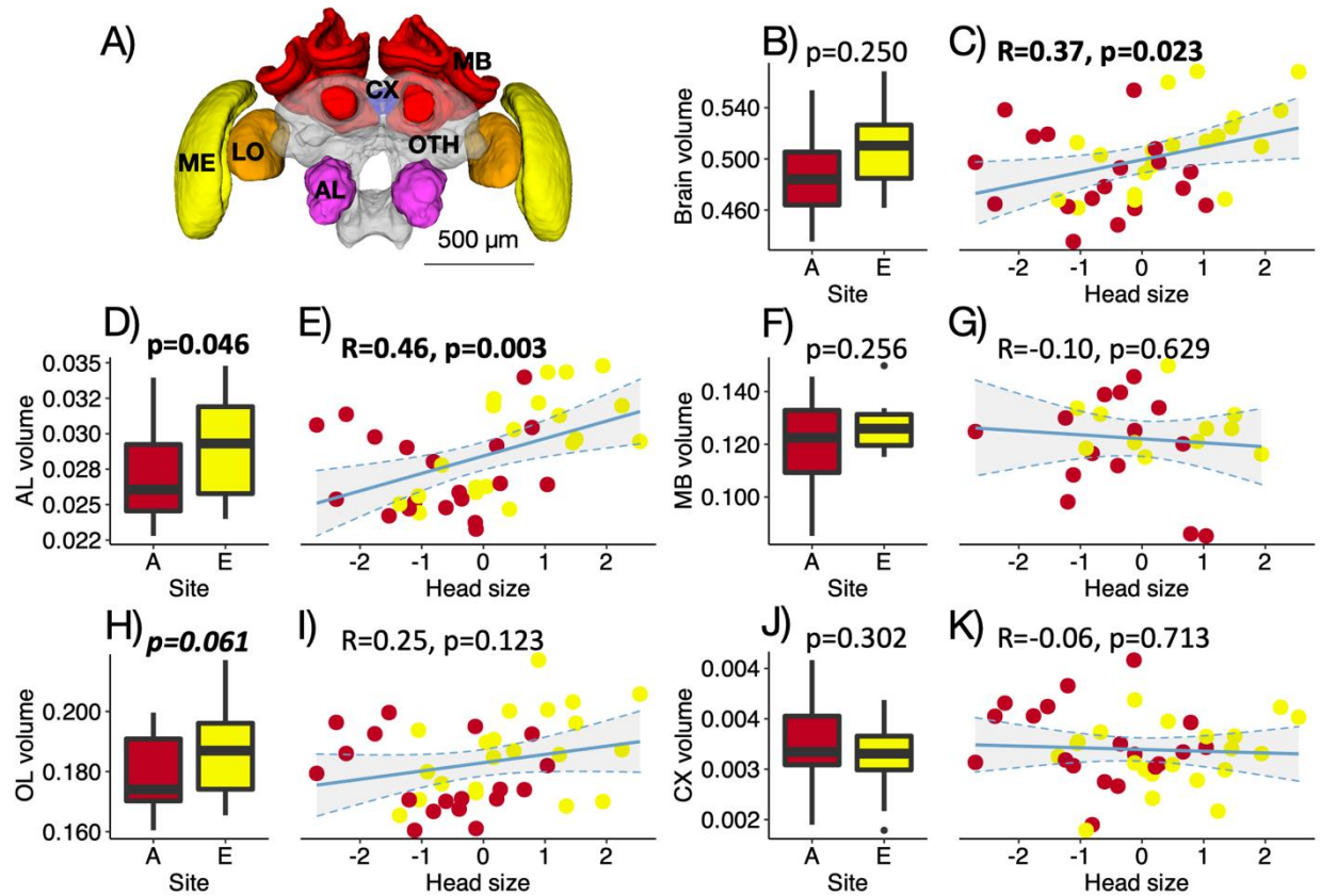
Figure 5: Brain area volumes ( \text{mm}^3 ) of forager bees from site A and E. A) Example of a reconstructed brain (frontal view) showing ALs, MBs, OLs (combining ME and LO), CX. B)-C) Total brain in function of the site (B) and head size (C). D)-E) Antennal lobes (AL) in function of the site (D) and head size (E). F)-G) Mushroom bodies (MB) in function of the site (F) and head size (G). H)-I) Optic lobes (OL) in function of the site (H) and head size (I). J)-K) Central complex (CX) in function of the site (J) and head size (K). Statistical comparisons for the neuropil volume between sites (Site A: N=18 ; Site E: N=20 ) were obtained with p-values from LMM. Shaded areas show 95% confidence interval of the regression line (in blue). Pearson correlation coefficient (R) and p-value are given. Significant p-values are displayed in bold.
