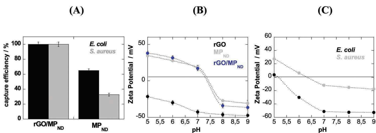
Figure 3.4: (A) Removal efficiency of MP ND and rGO/MP ND (500 mgmL -1 ) of E. coli and S. aureus ( 1 \times 10^9 cfu mL -1 ); (B) Zeta potential of rGO, MP ND , and rGO/MP ND as a function of solution pH; (C) Zeta potential of E. coli and S. aureus suspensions ( 1 \times 10^9 cfu mL -1 ).
