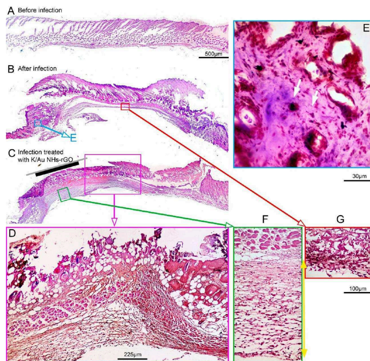
Figure 2.12: Histological analysis of mouse skin with longitudinal section across the wound and scar tissue. (A) Skin before infection. (B) Skin after infection. (C) Skin after infection with photothermally treated part of wound. (D) Interface between irradiated and nonirradiated tissue clearly showing abundant formation of granulation tissue beneath the heated area; (E) leukocyte and bacterial infiltration at the edge of the wound, where the tissue still was not converted to pus; (F and G) heated and unheated areas of infection demonstrating granulation tissue (marked with yellow arrow) attributable to wound healing, located beneath the layer of muscle (aligned at the top, to the same scale). Heated area shows viable muscular fiber and abundant granulation tissue, while the nonheated area possesses necrotic muscular fibers and puslike infiltrate beneath it. (A–C) H&E staining. (D–G) Gram staining. D–G are corresponding enlarged areas of parallel slides indicated by color.
