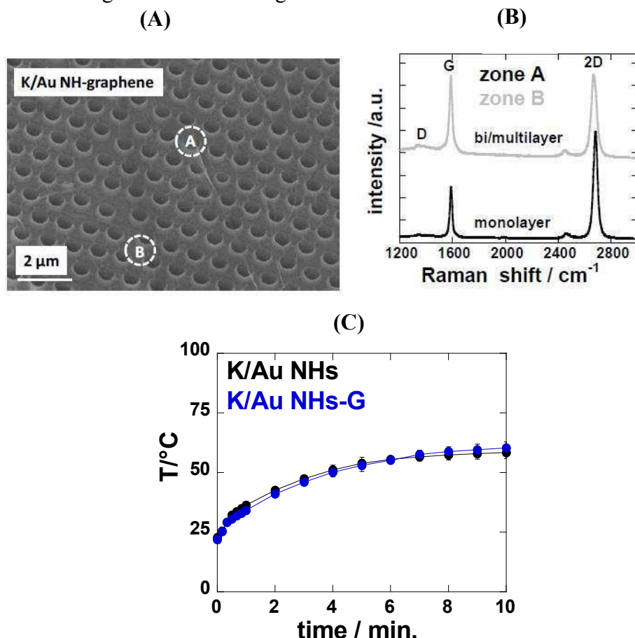
Figure 2.4: (A) SEM of graphene coated K/Au NHs; (B) Raman images on two different areas of K/Au NHs-graphene; (C) Photothermal heating curves of K/Au NHs (black) and K/Au NHs-G (blue) when immersed in water and exposed to laser light of 980 nm for 10 min at 2 W cm -2 .
