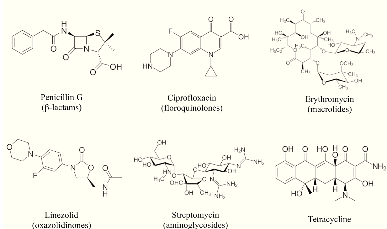
Figure 1.2: Chemical structures of typical antibiotics and their classes (in round brackets).
