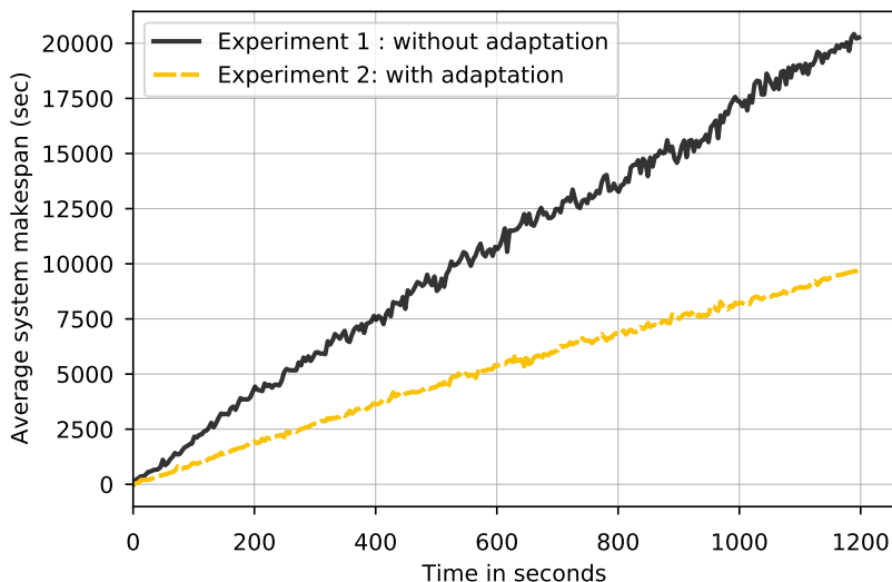
Figure 6.4 – With 19 data sources, the system makespan with data adaptation in experiment 2 is lower than in experiment 1, where no trade-off solution is used.
