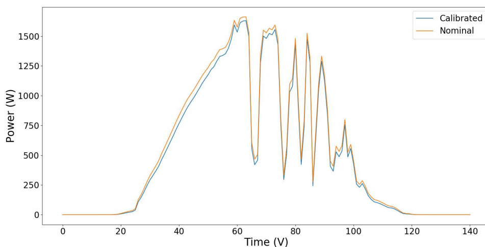
Figure 5.14: Comparison of the PV production with the calibrated and nominal parameter values.
