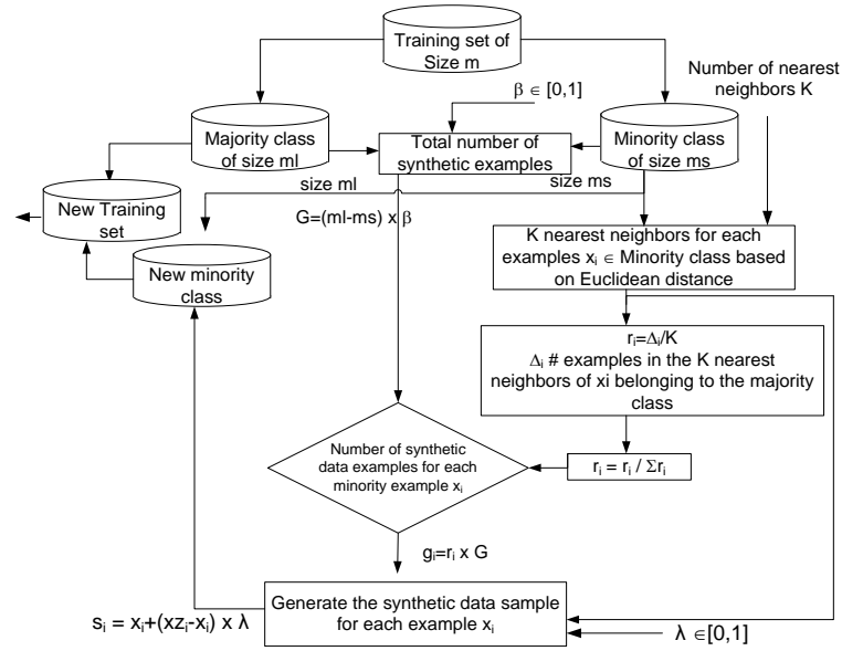
Figure 5.31. ADASYN flowchart.
