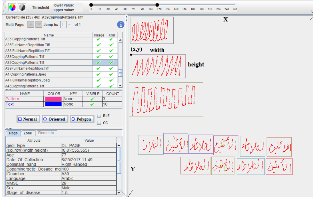
Figure 4.6. GEDI interface.
