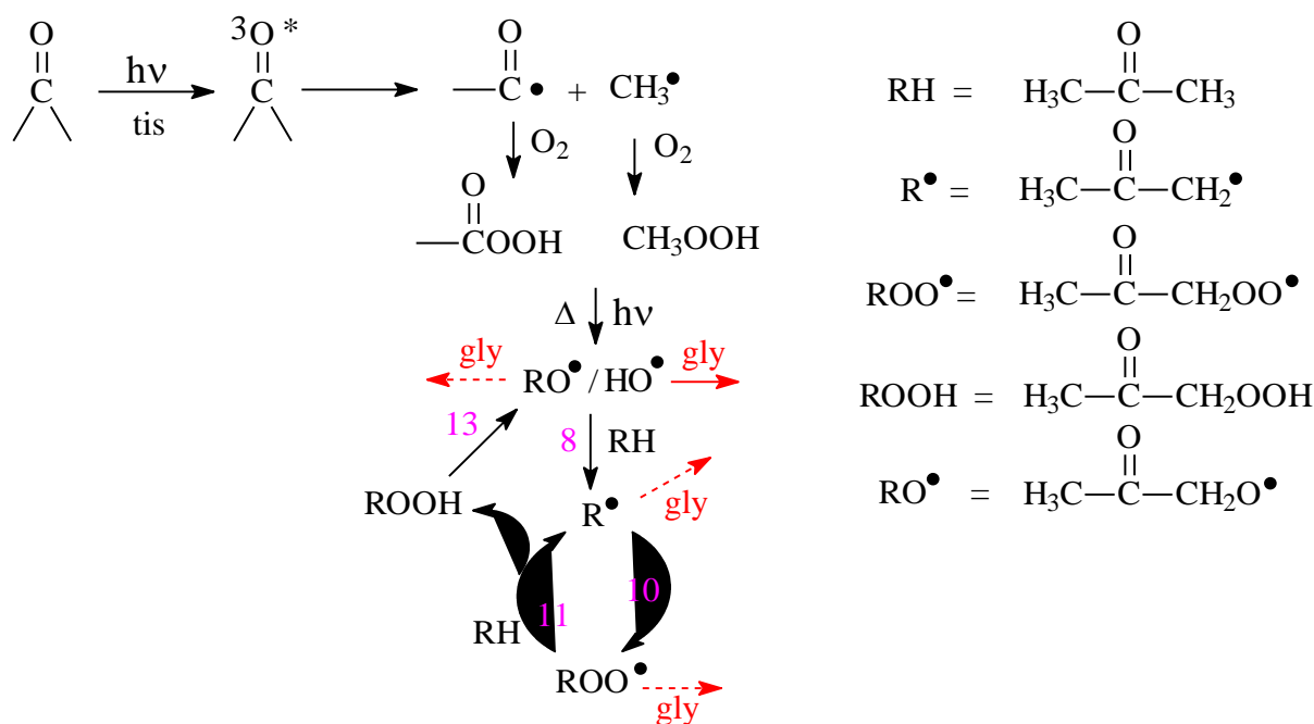
Scheme 1. Proposed mechanism of HO• formation upon irradiation of carbonyl compounds in presence of oxygen, and H-donor molecules RH.
