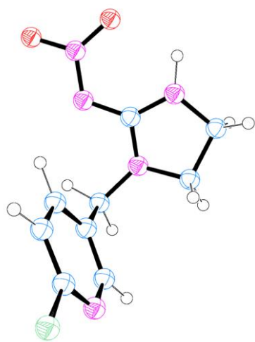
Global min in S_0 , ^1\text{RNNO}_2 (a) 0.0 kcal mol ^{-1}
