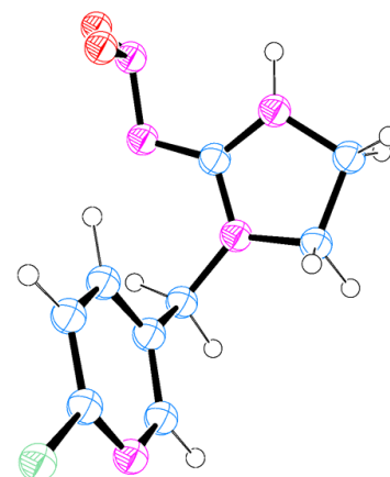
Min in T_1 , ^3\text{RNNO}_2 (c) 67.3 kcal mol ^{-1}
