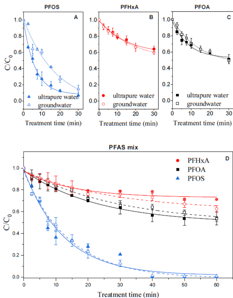
Figure 6. Degradation of pefluorooctanesulfonic acid (PFOS) (A), perfluorohexanoic acid (PFHxA) (B) and perfluorooctanoic acid (PFOA) (C) treated individually in ultrapure and groundwater matrices. Degradation of perfluoroalkyl substances (PFAS) treated in mixture (D) in ultrapure (solid symbols, solid lines) and groundwater (open symbols, dashed lines).
