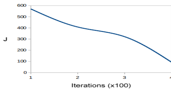
Figure 4.9: Convergence history
