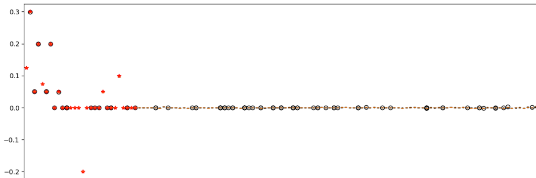
Figure A.40: Distribution of the parameters of the aggregators of an HCI with CG aggregators, trained on all 128 corners of the unit hypercube, with the standard flat model as the ground truth.
