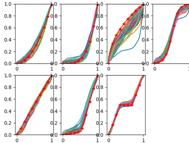
Figure A.48: Marginal utilities of 50 random UHCIs (random hierarchy) trained on data generated by the standard tree model, in regression setting, over 3000 data points.
