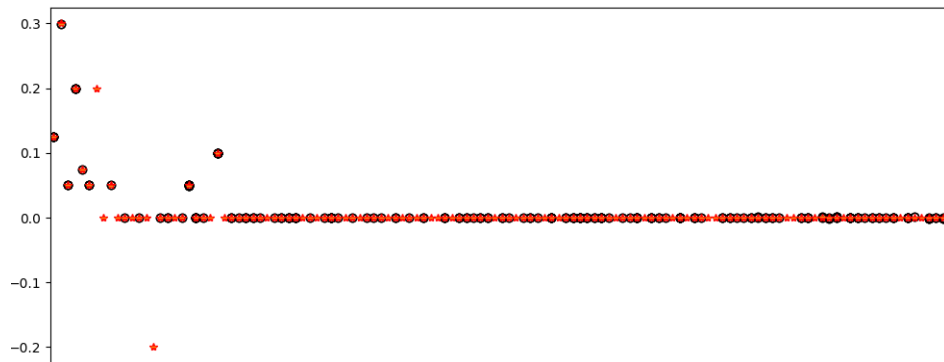
Figure 9.7: Distribution of the parameters of the aggregators of a CI with CG aggregators, 10,000 training examples generated by an HCI with 2-additive aggregators. 50 models trained in regression setting.
