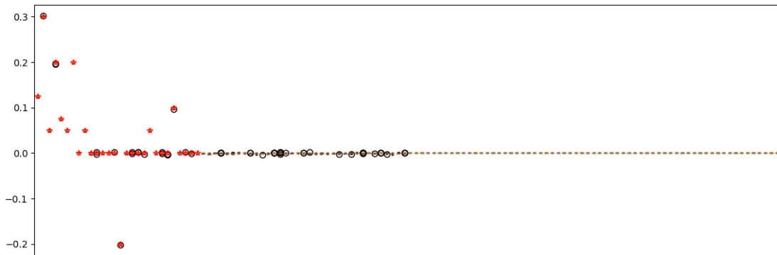
Figure 9.24: Distribution of the parameters of the aggregators of a CI with C3 aggregators, trained on the 62 corners of the unit hypercube with at most 3 coordinates set to 1. The labels are computed by the standard flat model.
