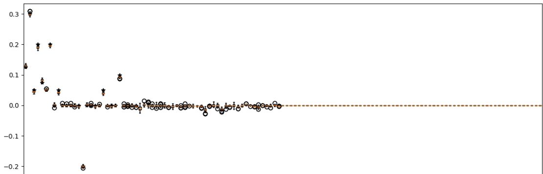
Figure A.16: Distribution of the parameters of the aggregators of a CI with 3-additive aggregators, 300 training examples generated by a flat 2-additive CI. 50 models trained in regression setting.
