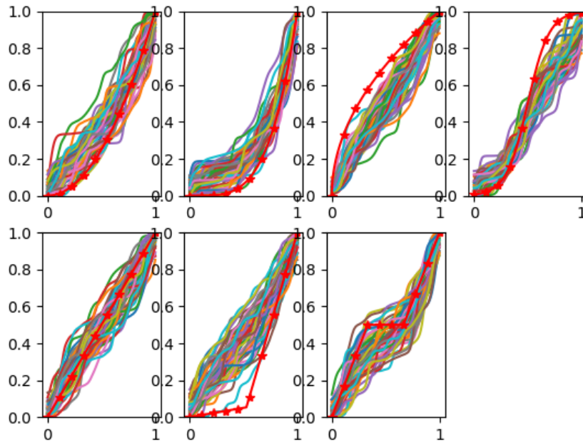
Figure A.15: Plotting the marginal utilities of 50 models trained in regression setting, 30 training examples generated by a UHCI. The aggregators are 2-additive.
