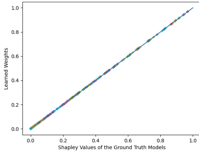
Figure 9.31: Plotting the learned weights of the linear models against the Shapley value of the generator CI model for the same criterion. The plot of y = x is also shown.
