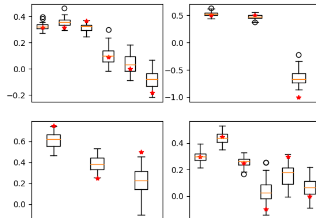
Figure A.28: Learned parameters of 50 2-additive HCI models trained on binary classification data generated by a 2-additive HCI. The training set was composed of 300 examples, with a noise level of 0.05.
