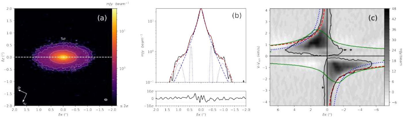
Fig. 1. (a) Continuum map at 232 GHz in logarithmic scale. White dotted contours show the 5, 10, 30, and 200 \sigma levels ( \sigma=50 \mu\text{Jy/beam} ). The white dashed line shows the disk major axis at PA=25.7°. (b) Continuum intensity profiles: Cut along PA=25.7° (in black) and deprojected and azimuthally averaged (in red). The tapered power law central component and the two Gaussian components, derived from the fitting and before beam convolution, are shown in blue dashed and dotted lines, respectively. Bottom panel shows the fit residuals and \pm 5\sigma limit (dotted lines). (c) Position-velocity diagram in 13 CO along PA= 25.7° in a pseudo-slit of 4'' width. The 3 \sigma contour is shown in black. The curves show maximum expected line-of-sight velocities V_{\text{max}} for three different models: a thin disk in Keplerian rotation around M_{\star} = 1.1M_{\odot} at an inclination of i = 63^{\circ} (red dashed line), pure rotation with constant angular momentum V_{\text{max}} \propto 1/r (blue dotted line), and a rotating and infalling bipolar shell (see Sect. 3.2.2) with Rd=300 au, \theta_0 = 70^{\circ} at an inclination of i = 63^{\circ} (green solid line).
