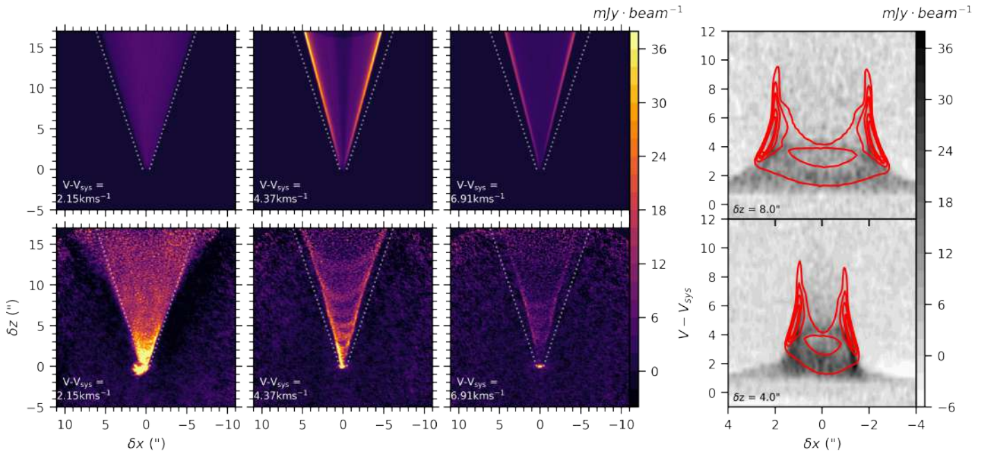
Fig. 10: Left panels: Individual ^{12}\text{CO} channel maps computed from the global disk wind model at selected line of sight velocities (top row) and compared to observations (bottom row). The color scale is the same for all the channel maps. Right panels: Position-Velocity diagrams at two positions along the flow and averaged over a slice of \Delta Z = 0.2'' . The background greyscale image shows the observations and the red contours trace predictions from the disk wind model.
