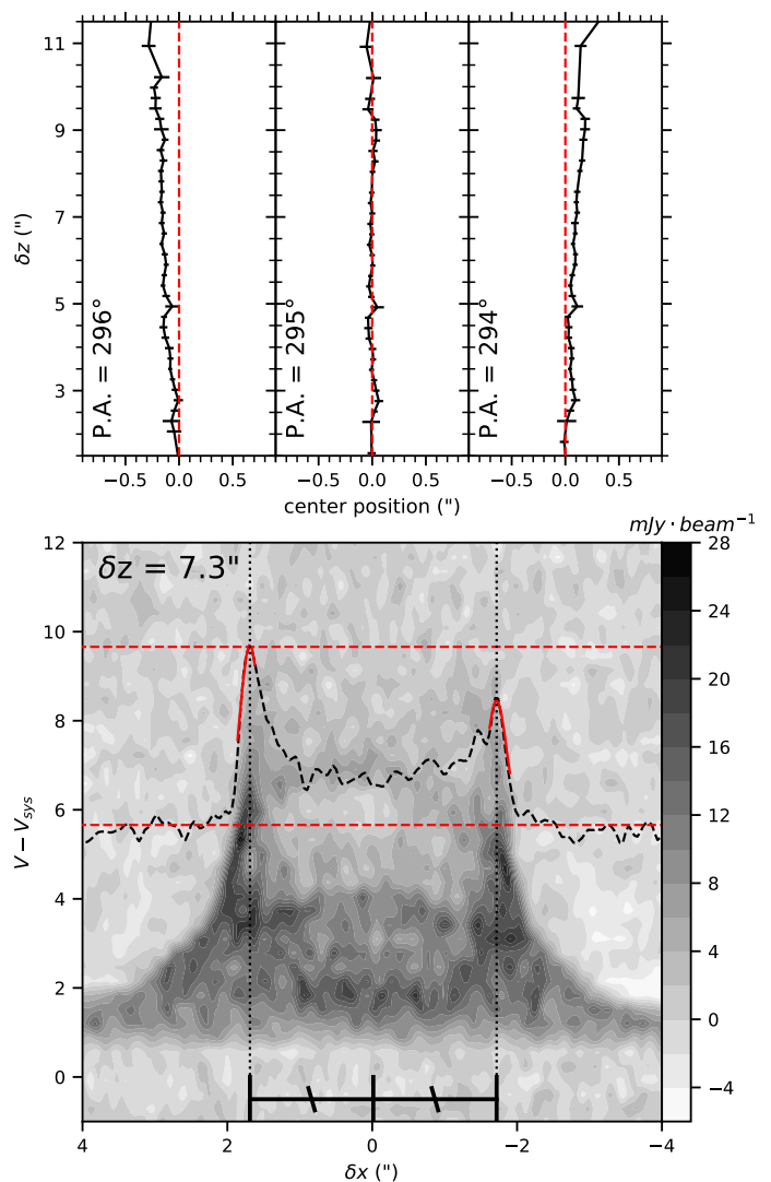
Fig. A.1: Top panels: Determination of the high-velocity component radial center as a function of projected heights above the disk for different P.A. orientations. Bottom panel: ^{12}\text{CO} PV diagram perpendicular to the outflow axis. The black dashed profile shows the emissivity integrated from the PV diagram between (V - V_{\text{sys}}) = 6.64 \text{ km s}^{-1} to (V - V_{\text{sys}}) = 9.77 \text{ km s}^{-1} . The red curves show Gaussian fits used to derive the radial positions of the two edge peaks. The average of these two radial positions give the radial center at this height.
