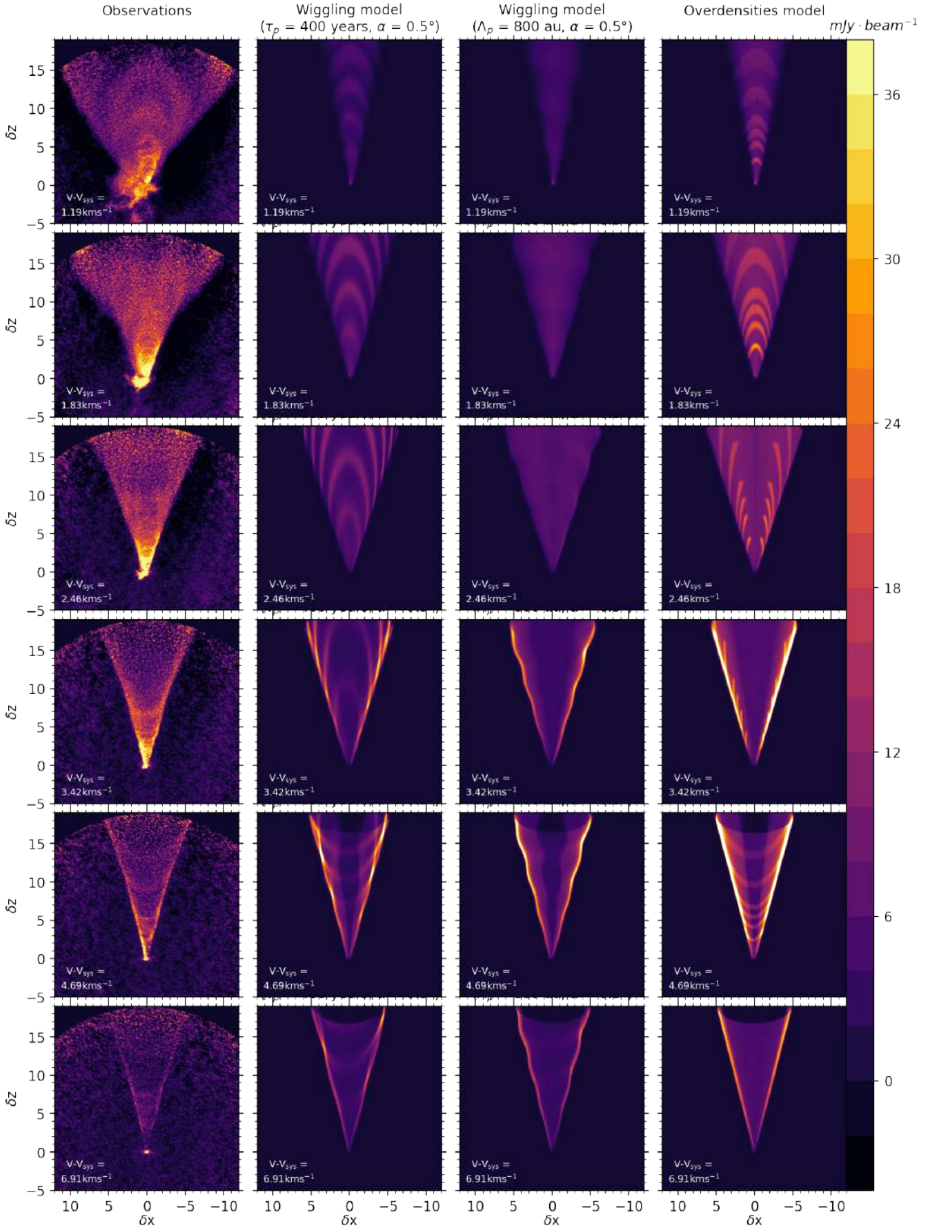
Fig. G.1: ^{12}\text{CO} observed (first column) and synthetic channel maps at selected line-of-sight velocities. The second and third columns correspond to the generic models with axis precession presented in Sect. 5.2. The last column corresponds to a disk wind model with density enhancement, as presented in Sect. 5.3
