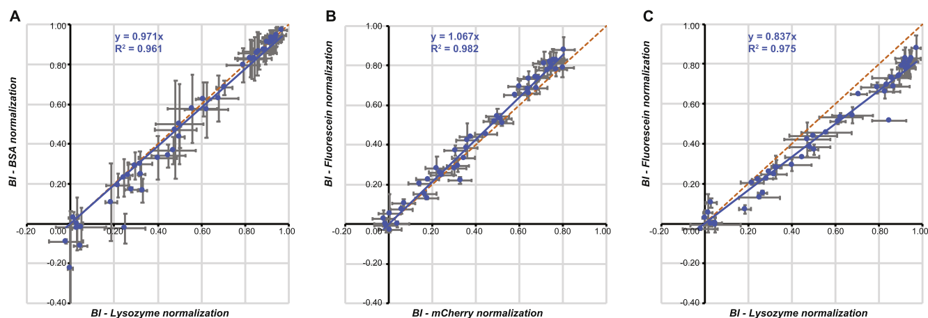
Fig. 5. Comparison of holdup binding intensities (BI) normalized by four internal markers. The holdup assay can be performed using either capillary electrophoresis or fluorescence spectroscopy for quantification of unbound analyte. For each approach, two alternative internal markers were tested. When the analyte was quantified by capillary electrophoresis, lysozyme and BSA were used for normalization (A). Note the high correlation between BI normalized by lysozyme and by BSA. When the analyte was quantified by tryptophan fluorescence, the internal markers were mCherry and fluorescein (B). Finally, it is apparent from the scatter plot C that the BI (lysozyme) from capillary electrophoresis are higher than the BI (fluorescein) that were obtained by measuring fluorescence. The plotted BI values are the mean of duplicated experiments with standard deviation shown as error bars. The linear regression line is plotted on each graph and its equation with coefficient of determination R^2 are indicated in the top left corner. The function y = x is plotted in dotted orange line on each graph. (For interpretation of the references to color in this figure legend, the reader is referred to the Web version of this article.)
