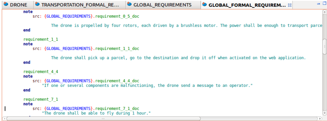
Figure 3.9: Integration of documentations artifacts into code
