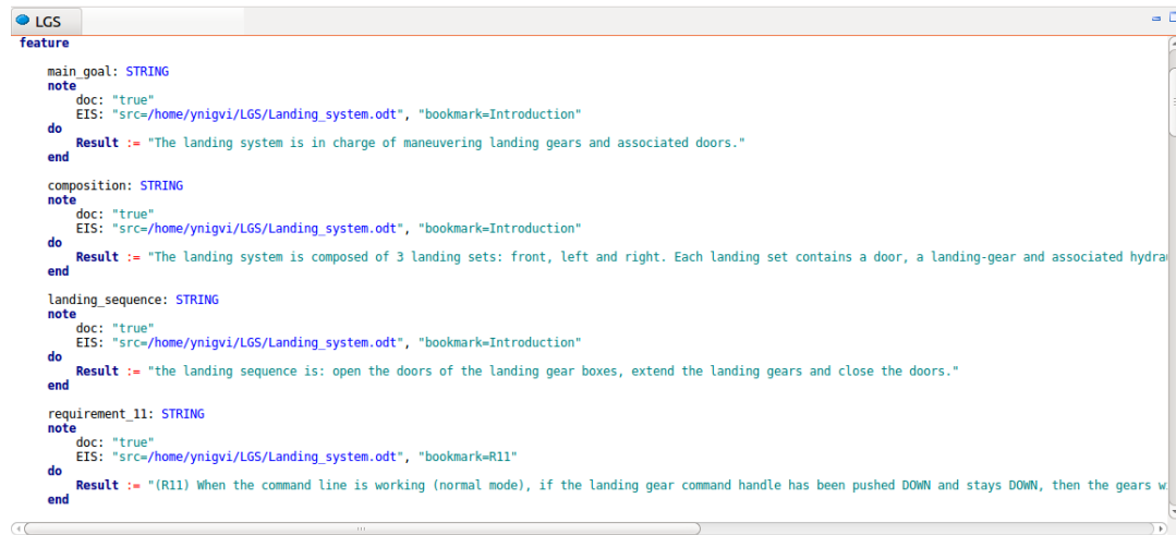
Figure 3.11: LGS requirements in Eiffel code
