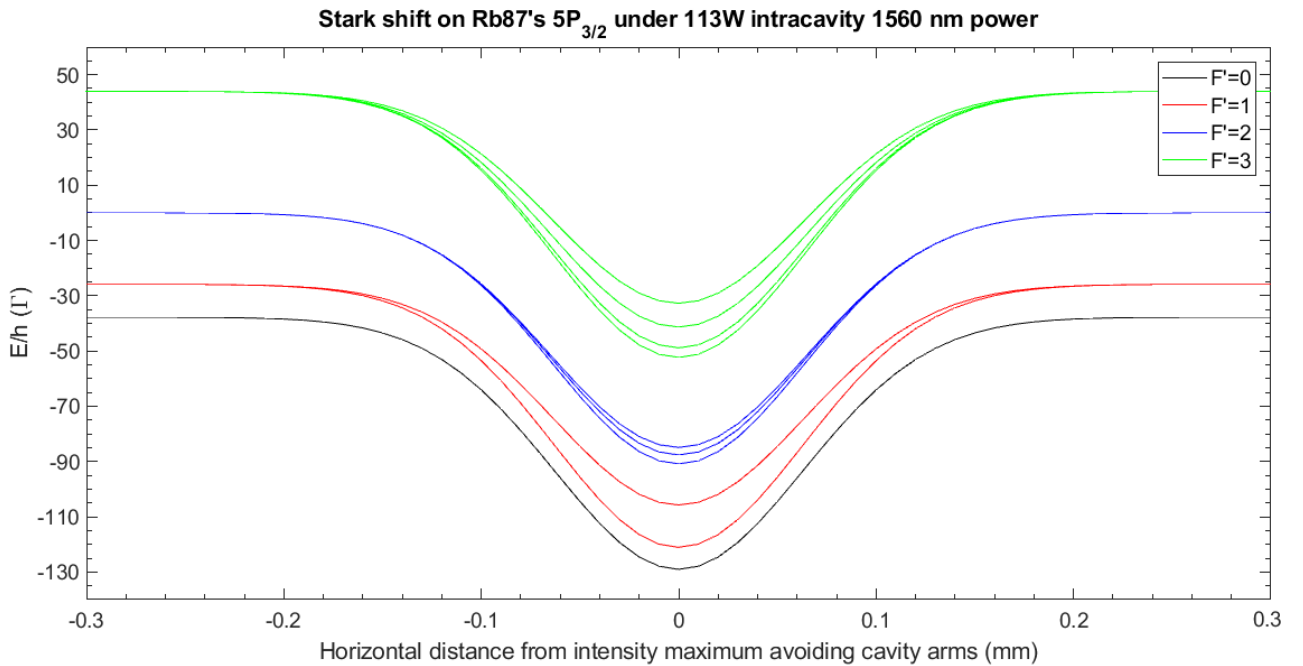
Figure 5.4: AC Stark shift on ^{87}\text{Rb} 's 5P_{3/2} manifold under 1560 nm FORT at trap depth of 700 \mu K, in units of the natural linewidth \Gamma and as a function of horizontal distance from the maximum intensity point. For energies, the origin has been chosen at the bare F' = 2 level, which is the level of interest for our gray molasses scheme.
