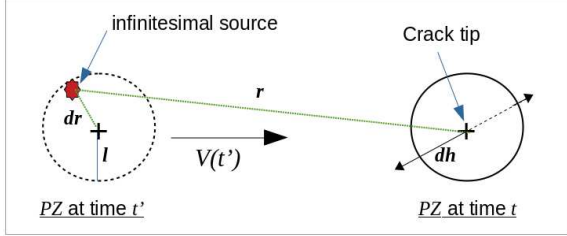
FIG. 1. Illustration of the geometric parameters used in Eq. (2). dh is perpendicular to the figure perspective.
