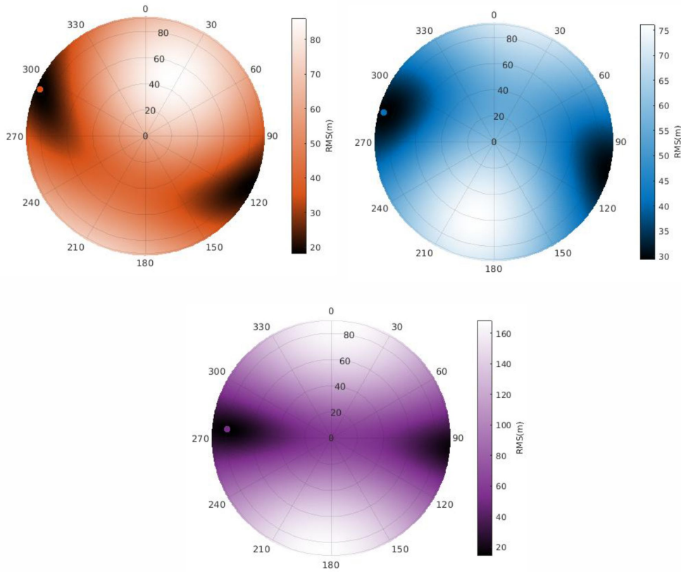
Figure 5.4 – Stereoplots showing the root mean square (RMS) of the orthogonal distance between the seismic events and a plane with varying orientation: dip from 0^\circ to 90^\circ and dip direction from 0^\circ to 360^\circ , in steps of 1^\circ . Orange: thermal stimulation, blue: injection interval hydraulic stimulation, violet: delayed interval hydraulic stimulation. The small colored circles show the orientation with minimum RMS.
