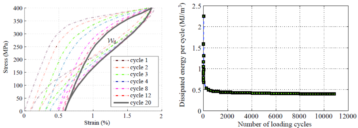
Figure 1-5: a) SE cycling for twenty cycles, b) dissipated energy per cycle versus the number of loading cycles (image taken from [19]).
