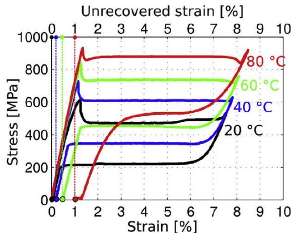
Figure 1-3: Superelastic response of a NiTi wire (image taken from [18]).
