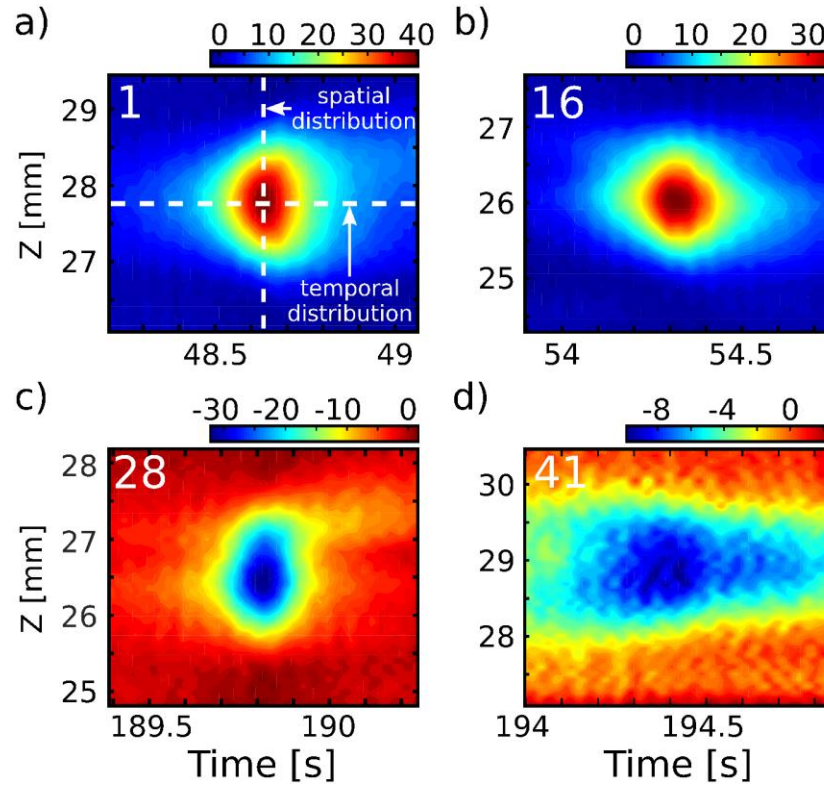
Figure 2-7 : Focus over different localized events: a, b) spatio-temporal color matrices of reconstructed localized heat sources in K \cdot s^{-1} related to martensite nucleation and merging events that appeared during loading at locations 1 and 16 as depicted in Figure 2-6d, respectively; c), d) same for austenite nucleation and merging events that appeared during unloading at locations 28 and 41 as depicted in Figure 2-6e, respectively.
