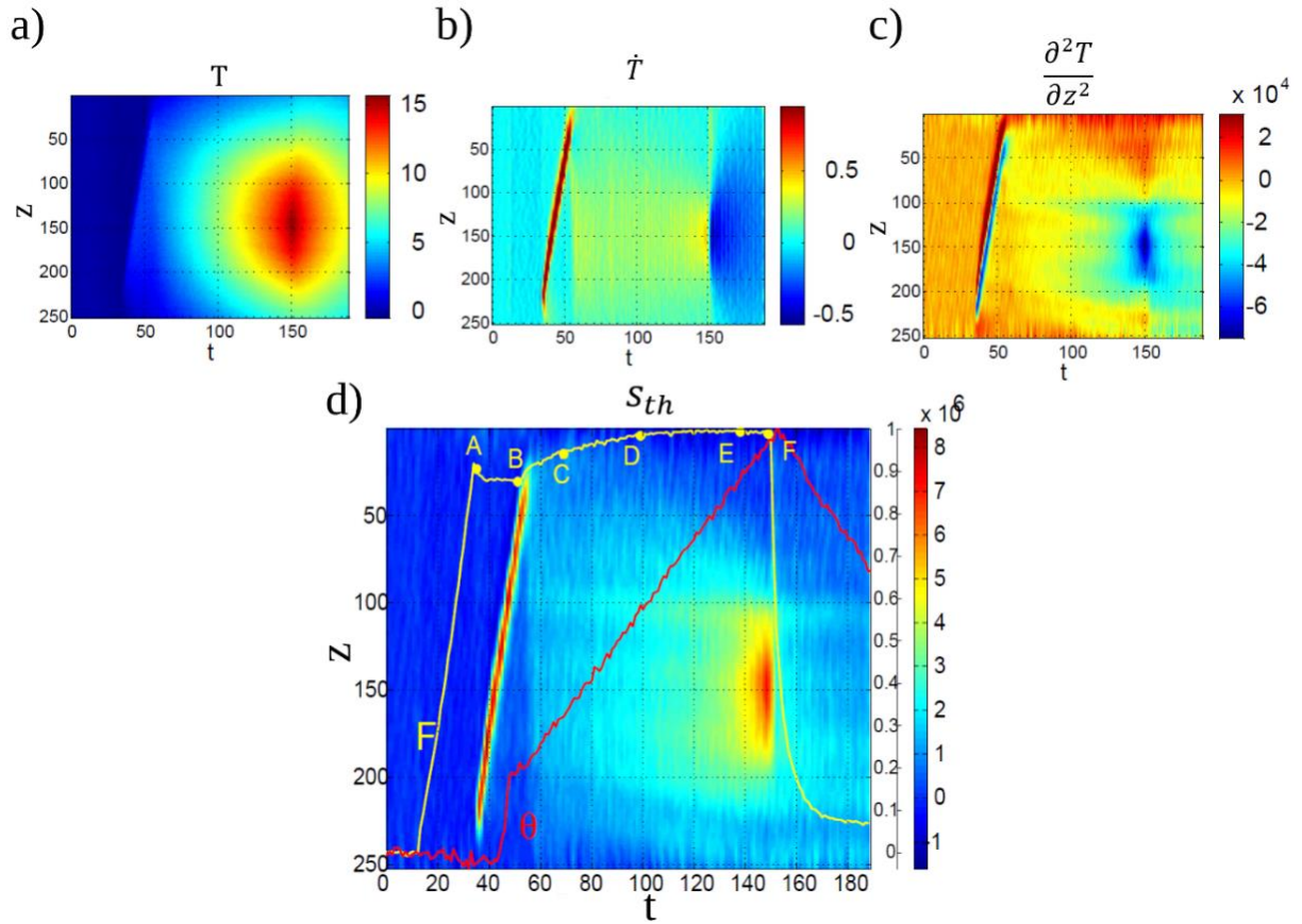
Figure 1-33: Example of 1D heat source reconstruction for a tensile test on S322MC steel: a) experimental thermal variation [K], b) first-order time derivative [ K.s^{-1} ], c) second-order spatial derivative [ K.m^{-2} ], d) heat source field [ W.m^{-3} ] (adapted from [90]).
