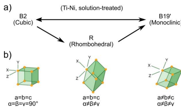
Figure 1-1: a) Transformation path in NiTi SMAs (adapted from [2]) and b) crystal lattices of different phases (adapted from Encyclopedia Britannica, Inc).
