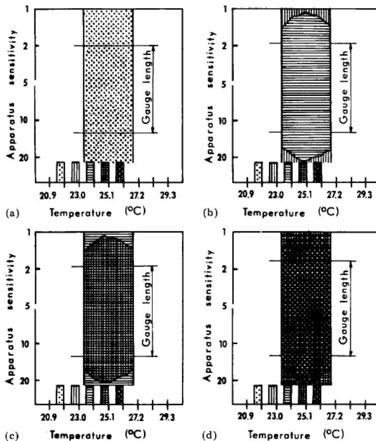
Figure 1-24: Temperature distribution on the surface of steel specimen: a ) before elongation, b ) after 19 s of elongation, c ) after 30 s of elongation, and d ) after 40 s of elongation (image taken from [83]).
