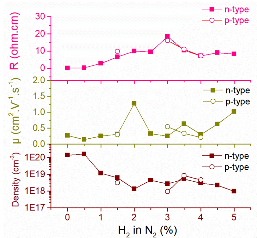
Figure II. 23: Resistivity ( R ), carrier mobility ( \mu ) and carrier density of \text{Zn}_{\text{DC}}\text{Sn}_{\text{RF}} series (determined from Hall effect measurements) versus \text{H}_2/\text{N}_2 ratio.
