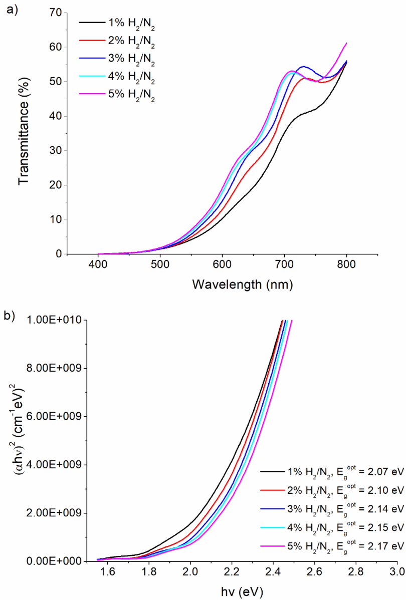
Figure II. 24: a) Transmittance vs. wavelength spectra (UV-Vis spectroscopy) for Zn_{DC}Sn_{RF} samples deposited under varied H_2/N_2 ratios sputtering atmospheres, b) Corresponding optical bandgap values calculated using Tauc's equation.
