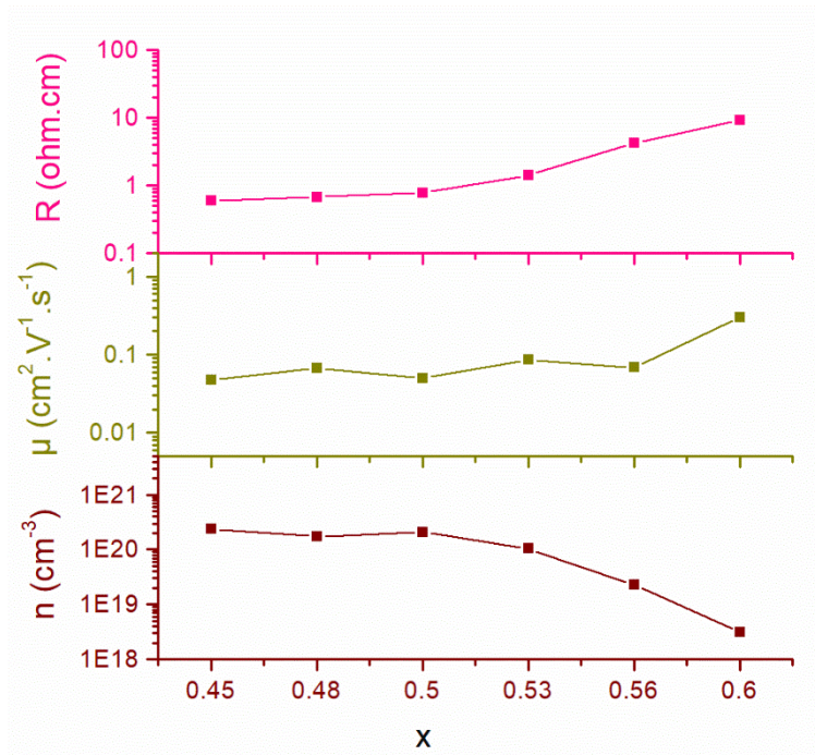
Figure IV. 16: Resistivity (R), carrier mobility (μ) and carrier density (n) of Zn x Sn 1-x N 2 thin films (Zn DC Sn DC series) with 0.45 \leq x \leq 0.60 .
