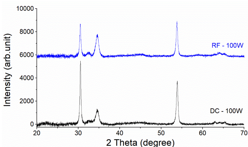
Figure IV. 25: XRD diffractograms of ZnSnN_2 deposited in DC mode ( ZnSn_{DC} sample) and RF mode ( ZnSn_{RF} sample) from a compound target.
