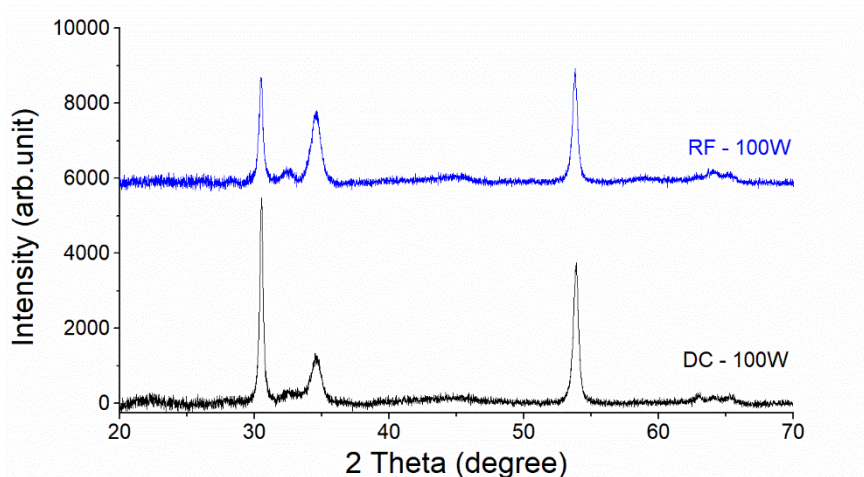
Figure IV. 25: XRD diffractograms of ZnSnN_2 deposited in DC mode ( ZnSn_{DC} sample) and RF mode ( ZnSn_{RF} sample) from a compound target.
