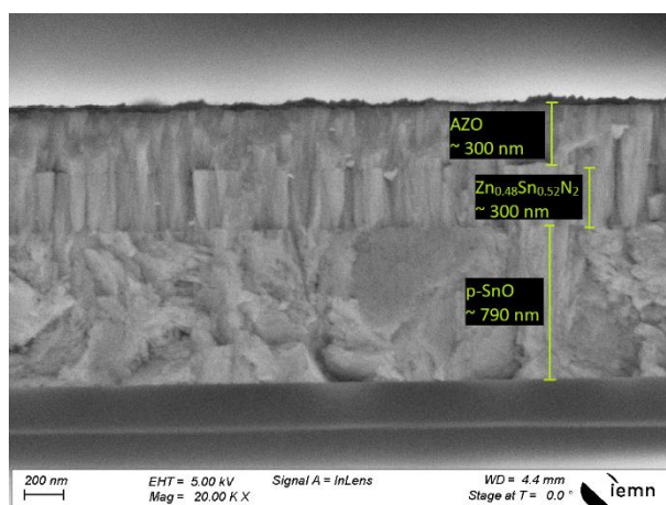
Figure VI. 24: Cross-section SEM image of p\text{-SnO}/\text{Zn}_{0.48}\text{Sn}_{0.52}\text{N}_2/\text{AZO} with sputtering time of SnO increased to 27 min, and \text{ZnSnN}_2 was deposited in \text{Zn}_{\text{DC}}\text{Sn}_{\text{RF}} mode (Structure2.4).
