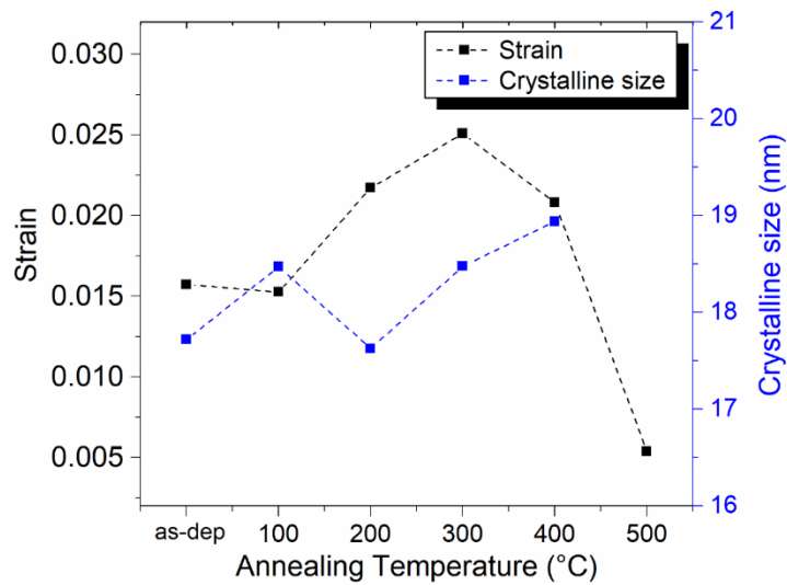
Figure III. 31: Strain and crystal size of (200) plane of \text{Zn}_{\text{RF}}\text{Sn}_{\text{DC}}\text{RF}_{\text{Zn}}\text{DC}_{\text{Sn}}\text{-NA} thin films on Eagle XG substrate after annealing from 100^\circ\text{C} to 500^\circ\text{C} .
