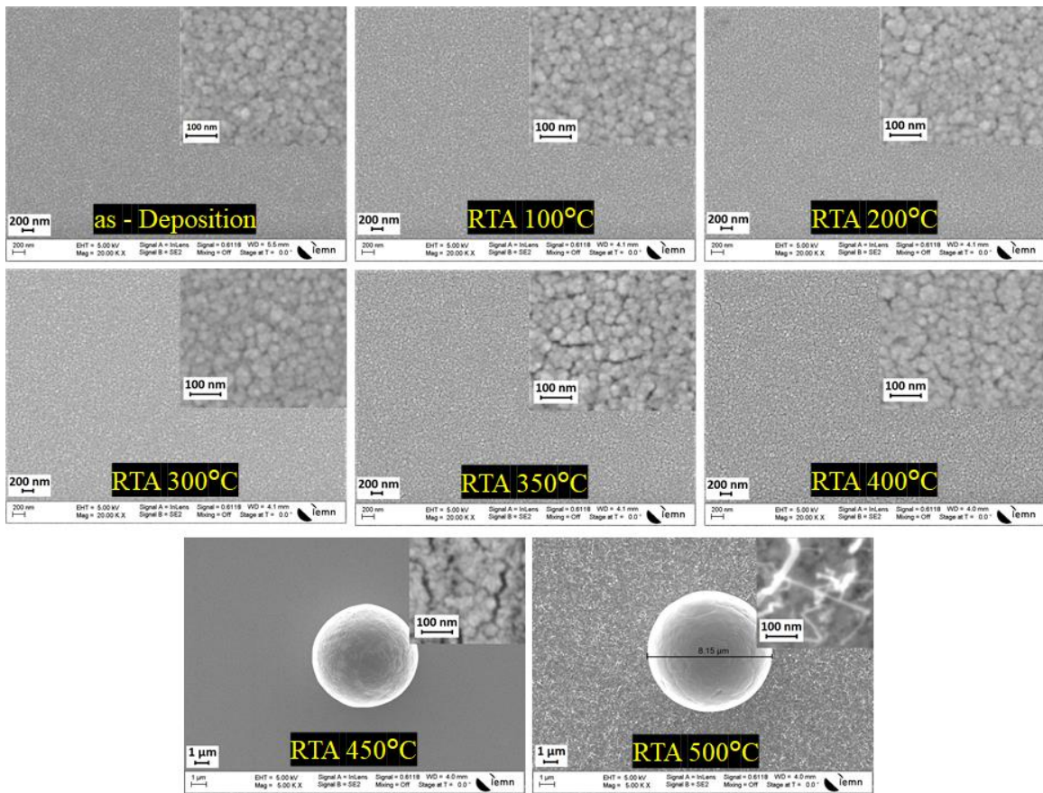
Figure III. 19: SEM images of Zn_{DC}Sn_{RF} -NA thin films on Si (100) after RTA treatment (the scale of 450° and 500°C sample images is 4 times greater compared to others).
