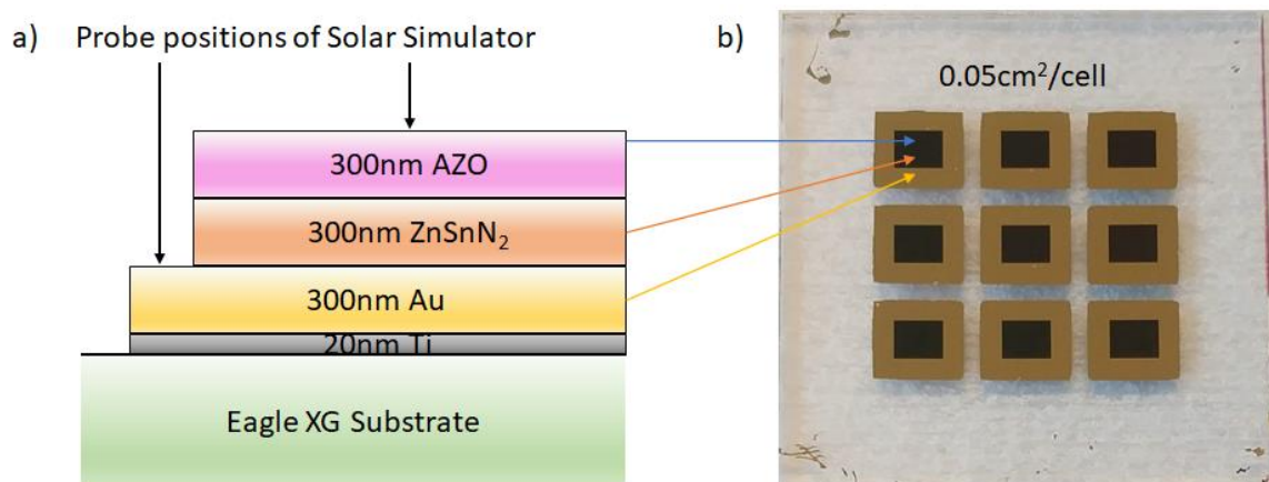
Figure VI. 6: a) Cross-section and b) Final view of Structure1.2 devices (0.05cm 2 cells).
