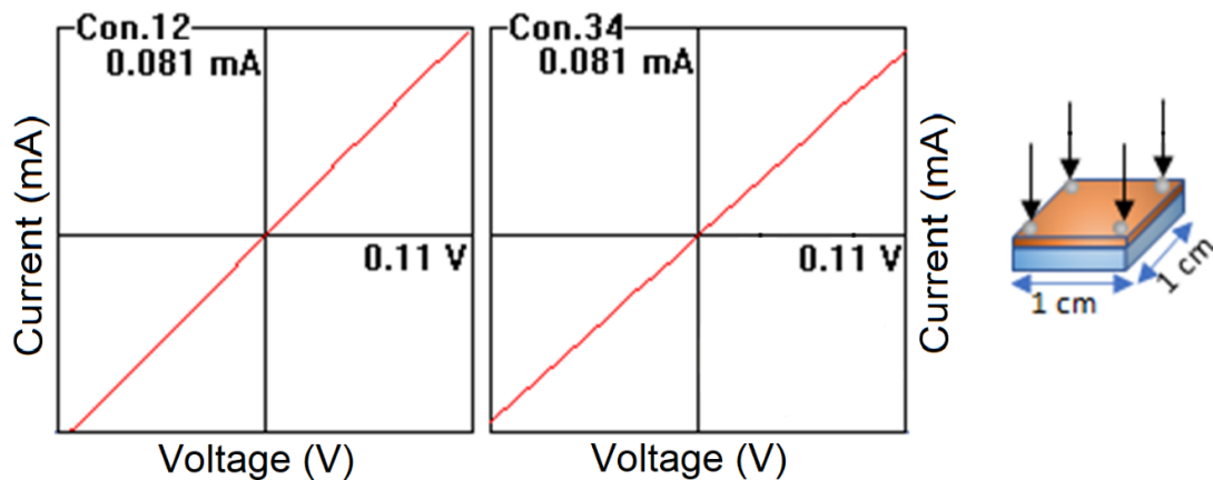
Figure II. 8: I-V curves obtained from Van Der Pauw resistivity measurements of sample N 2 /Ar = 2.5 (insert shows the way contacts are taken).
