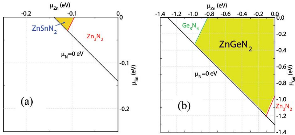
Figure I. 8: The yellow regions provide stabilized single-phase \text{ZnSnN}_2 (a) and \text{ZnGeN}_2 (b), obtained by calculated chemical potentials of the component elements ( \mu_{\text{Zn}} , \mu_{\text{Sn}} , \mu_{\text{Ge}} , \mu_{\text{N}} ) [26].
