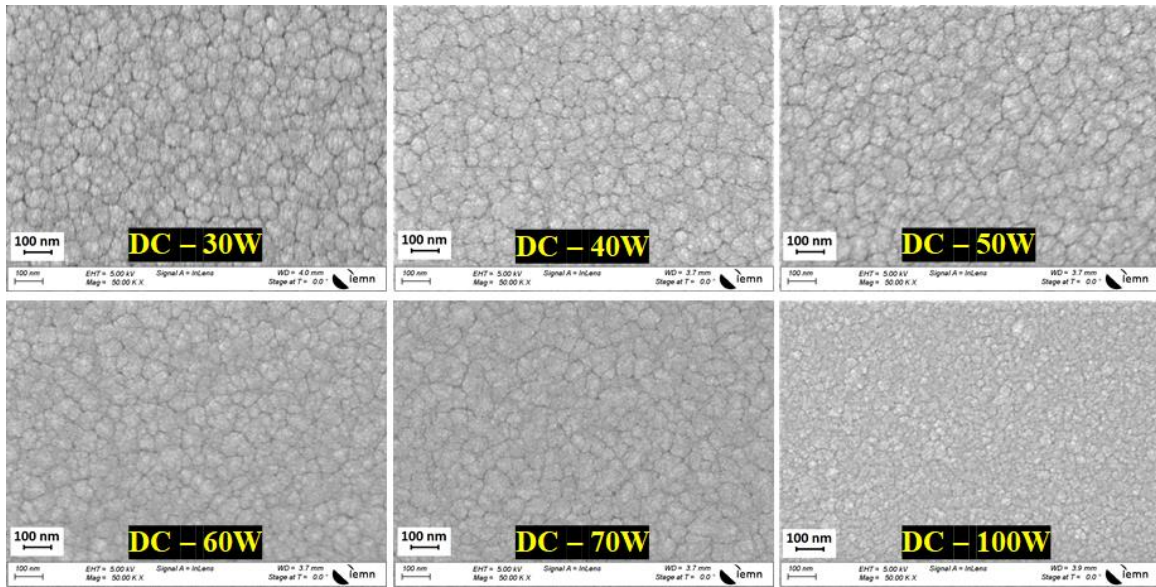
Figure IV. 19: Top-view SEM images of the Zn_xSn_{1-x}N_2 ( ZnSn_{DC} series).
