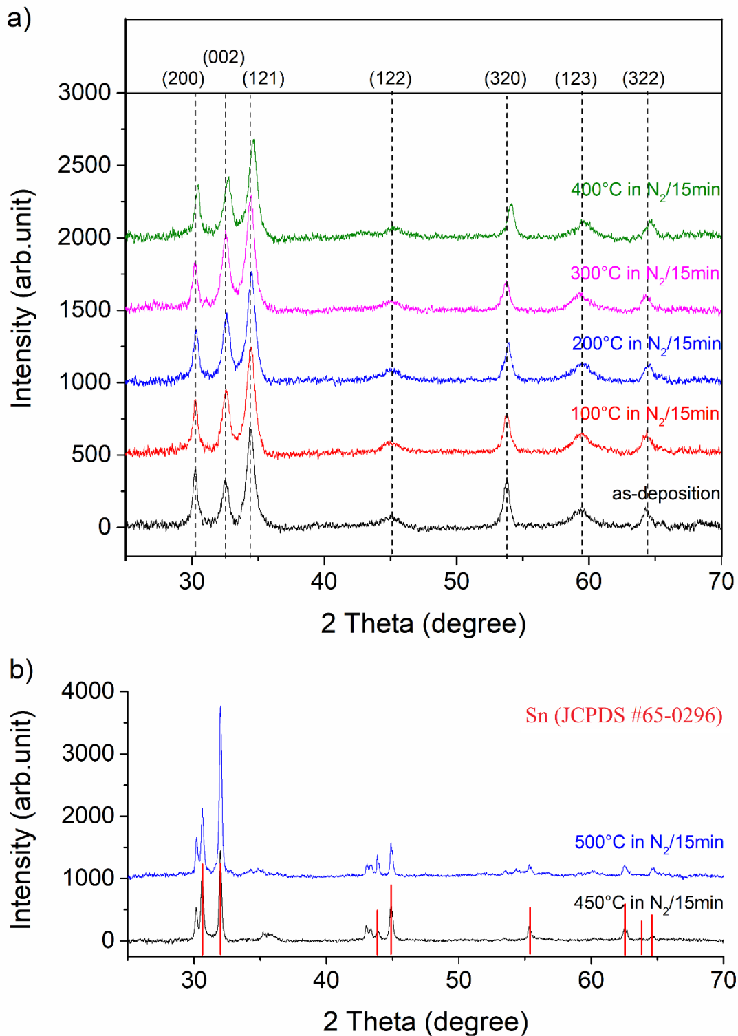
Figure III. 20: XRD diffractograms of ZnDCSnRF-NA thin films on Si (100) for different post-annealing temperatures: a) from 100°C to 400°C, b) 450°C and 500° data compared to XRD data of Sn on red peaks.
