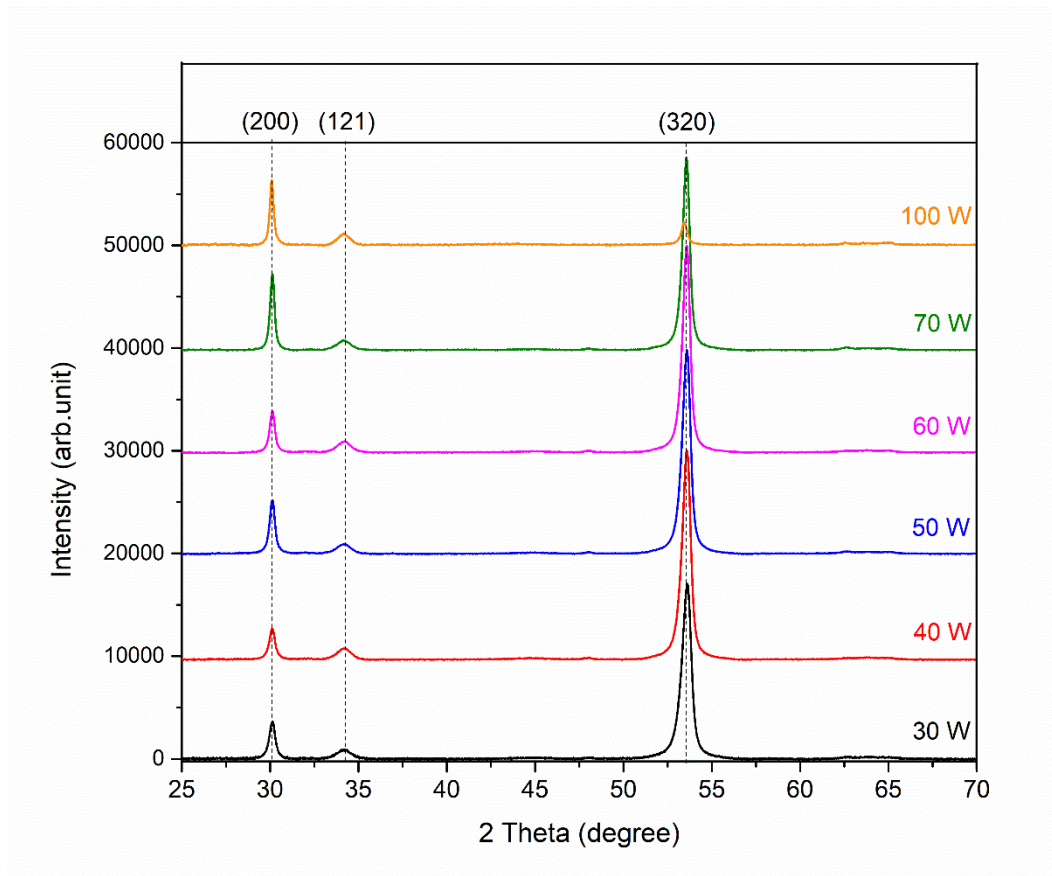
Figure IV. 20: XRD diffractograms of Zn_xSn_{1-x}N_2 thin films ( ZnSn_{DC} series) via DC power.
