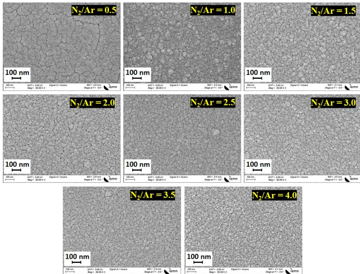
Figure II. 12: Top view of Zn_{RF}Sn_{DC} series deposited at different N_2/Ar ratios.
