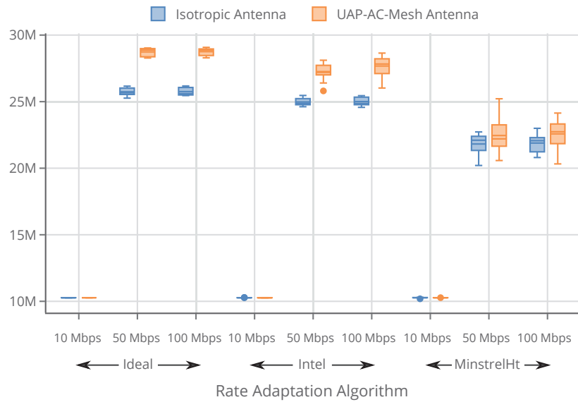
Figure 6.9: Comparison of the average received throughput per link for Scenario #2 with r = 100 m and 5 nodes.
