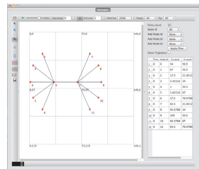
Figure 3.4: ns-3 NetAnim component, which can be used as an offline GUI for ns-3 simulations, replaying traces collected during simulation. Extracted from the project wiki.
