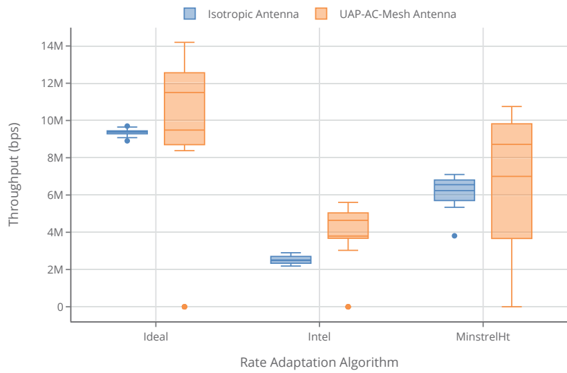
Figure 6.15: Comparison of the average received throughput at the sink for Scenario #3 with d = 1000 m, 5 nodes, and 20 random initial orientations with the 3 dBi directional antenna.
