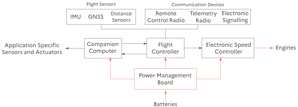
Figure 2.6: Generic architecture of a small multicopter drone.
