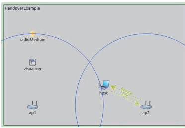
Figure 3.5: OMNeT++ and INET Framework GUI example, extracted from the Handover Example Animation from the OMNeT++ Website.
