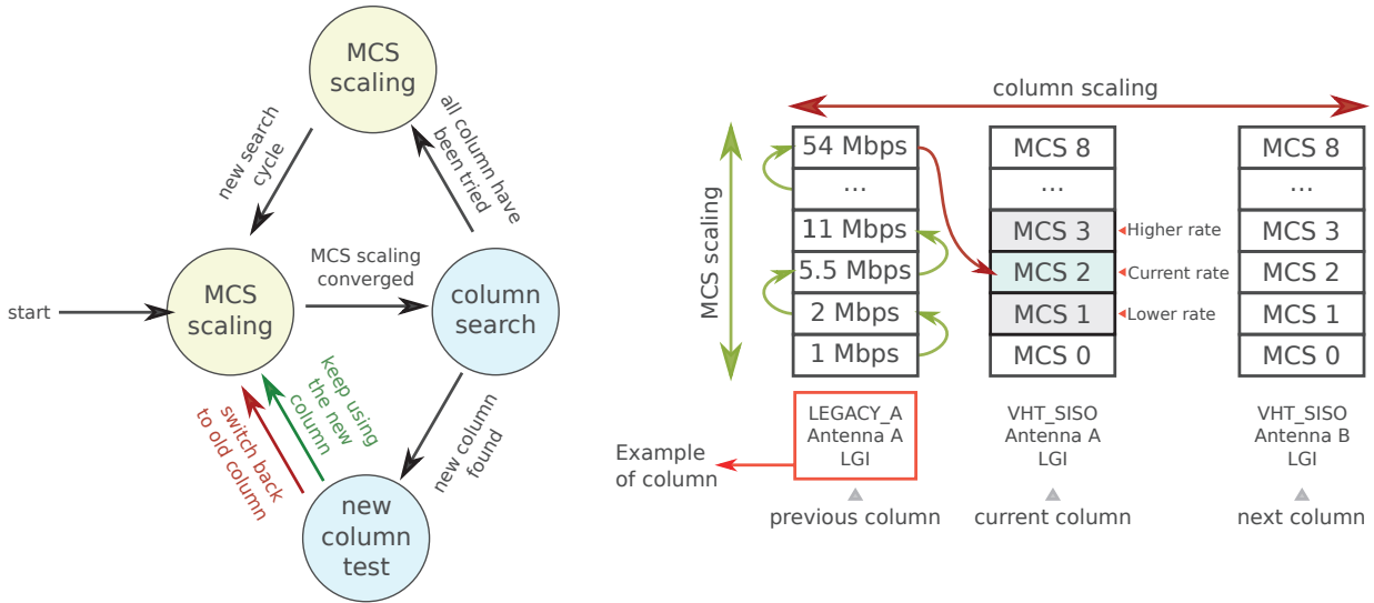
Figure 4.10: Flowchart of the different states of Iwl-Mvm-Rs (left) and example of sequence of decisions made by the Iwl-Mvm-Rs (right).
