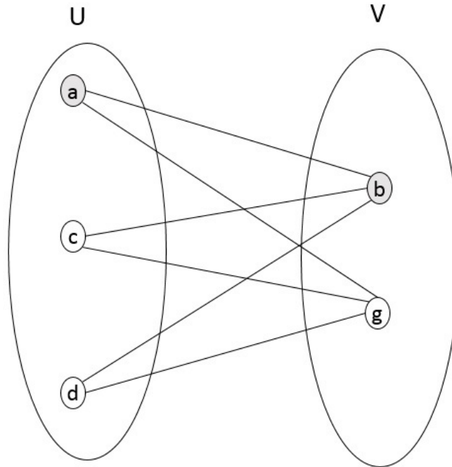
FIGURE 3.10 – graphe biparti
