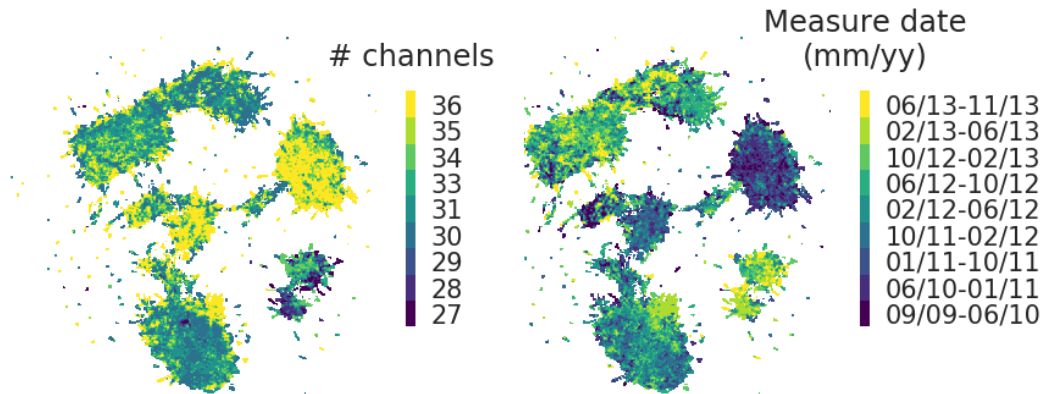
Figure 2.10 – Structure related to the original recording’s number of EEG channels and measurement date in TS-learned features on the entire TUAB dataset. The overall different number of EEG channels and measurement date in each cluster reveals that the cluster-like structure reflects differences in experimental setups. See Figure 2.7 for a description of how the density plots are computed.
