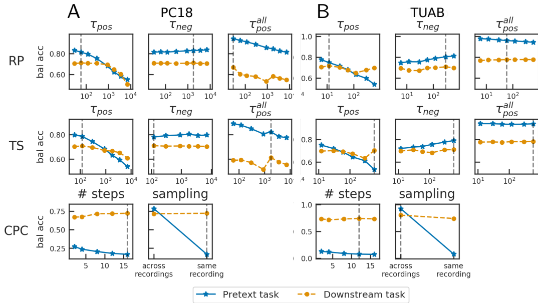
Figure 2.11 – Impact of principal hyperparameters on pretext (blue) and downstream (yellow) task performance, measured with balanced accuracy on the validation set of (A) PC18 and (B) TUAB. Each row corresponds to a different SSL pretext task. For both RP and TS, we varied the hyperparameters that control the length of the positive and negative contexts ( \tau_{pos} , \tau_{neg} , in seconds); the exponent “all” indicates that negative windows were sampled across all recordings instead of within the same recording. For CPC, we varied the number of predicted windows and the type of negative sampling. Finally, the best hyperparameter values in terms of downstream task performance are emphasized using vertical dashed lines. See text for more details on the hyperparameter search procedure.
