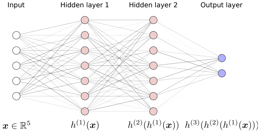
Figure 1.4 – A fully-connected neural network with two hidden layers. Edges represent weights between the output of a layer and units of the next layer. The opacity of the edges illustrate the relative weights of randomly initialized parameters. Adapted from LeNail (2019).
