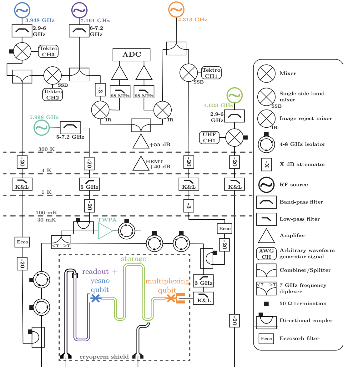
Figure b.2: Schematic of the setup. Each electromagnetic mode of the experiment is driven by a RF generator detuned by the modulation frequency and whose color matches the color of the corresponding mode in Fig. 5.1. Room temperature isolators are not represented for the sake of clarity.
