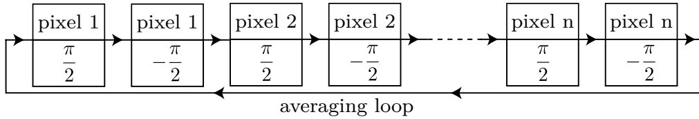
Figure c.2: Wigner tomography averaging. Each pixel of the Wigner function is measured twice (once with the \pi/2 pulse sequence and once with the -\pi/2 pulse sequence) before moving to the next pixel. Once all the pixels have been measured, we repeat the sequence to obtain the average.
