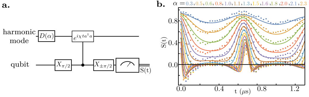
Figure c.3: Revival of the Ramsey interferences on the yes-no qubit a . Circuit diagram for Ramsey interferometry in the presence of harmonic mode photons. After displacement pulse, an unconditional \pi/2 pulse is applied to the qubit. We then let the qubit evolve freely during a time t before doing a new \pm\pi/2 pulse and measure its state. b . Measured (dots) and predicted (lines) signal S as a function of waiting time t for the storage mode and the yes-no qubit. Predicted signal is computed from Eq. (c.5). Yes-no qubit revivals occur every 2\pi/\chi_{s,\text{yn}} \approx 0.7\mu\text{s} .
