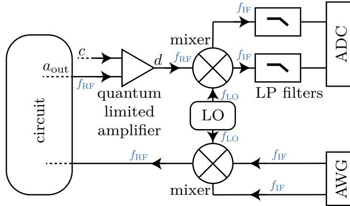
Figure 4.3: Scheme of a heterodyne measurement. An arbitrary waveform generator (AWG) emits an IF signal f_{IF} . The signal is up-converted using a mixer and an LO, generating a carrier at the frequency f_{LO} . The RF signal going out of the mixer is at the frequency f_{RF} = f_{LO} - f_{IF} . The RF signal is used to probe the circuit and the outgoing RF signal is amplified using a quantum-limited amplifier. The amplifier mixes and amplifies the mode a_{out} , which contains information about the circuit state with an idler mode b . The mode d going out of the amplifier is at the frequency f_{RF} . The signal is down-converted using the same LO and sent through low pass (LP) filters. The down-converted signal oscillating at the frequency f_{IF} is then digitized using an ADC. A final demodulation at the frequency f_{IF} is numerically performed.
