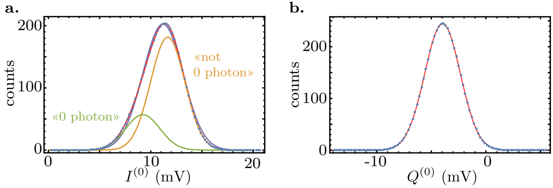
Figure 6.5: Histograms of the I^{(0)} and Q^{(0)} fluorescence records when measuring whether there are 0 photons when the storage mode is prepared in |\beta\rangle = |\sqrt{1.4}\rangle . a. The I^{(0)} histogram is composed of two Gaussian distributions corresponding to the “0 photon” (green line) and “not 0 photon” (yellow line) results. The red line is the sum of the two distributions. The purple line is a fit using only one Gaussian distribution. This single Gaussian distribution fit is not able to reproduce the shape of the distribution. Thus we reject the hypothesis that the I^{(0)} histogram is composed of a single Gaussian distribution. b. The Q^{(0)} histogram contains no information. It corresponds to a single Gaussian distribution (red line).
