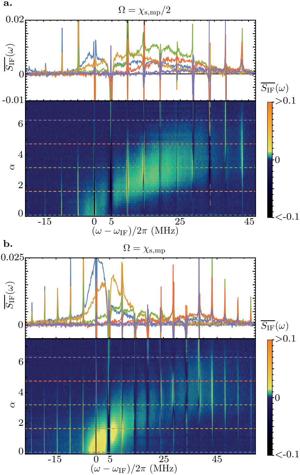
Figure 7.11: Measured normalized spectral density \overline{S}_{IF}(\omega, |\alpha|^2) as a function of the amplitude \alpha of the storage mode coherent state |\alpha\rangle . The drive strength \Omega is equal to a. \chi_{s,mp}/2 and b. \chi_{s,mp} . In each figure, the upper graph shows cuts of the lower graph for values of \alpha , indicated by the colored dashed lines.
