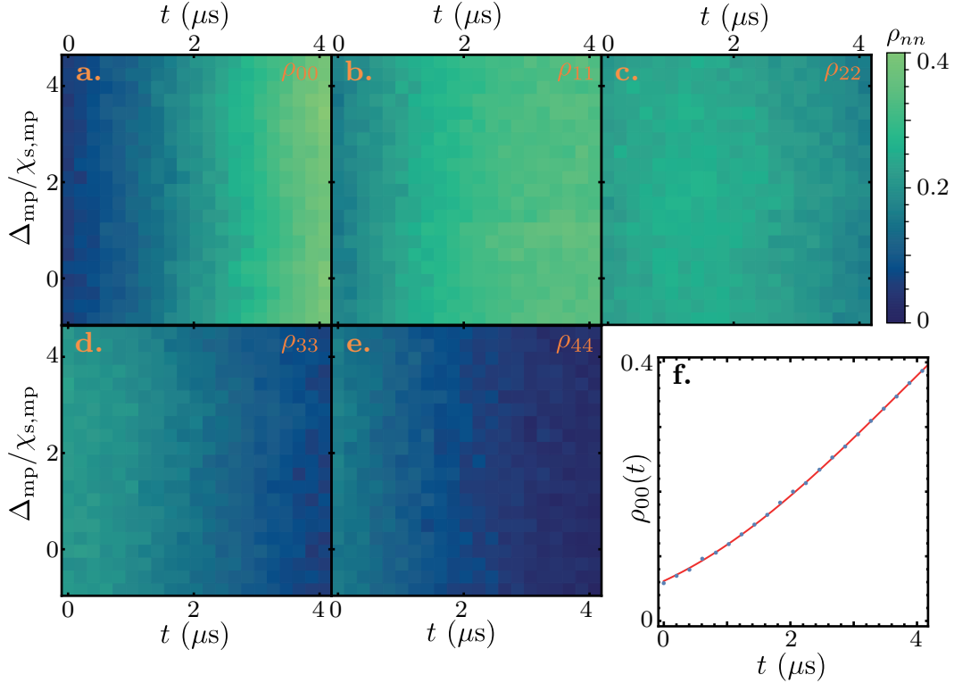
Figure 6.8: a. , b. , c. , d. et e. Diagonal element \rho_{nn} of the storage mode density matrix as a function of time t and detuning \Delta_{\text{mp}} . We check that the dynamics of the diagonal elements does not depend on \Delta_{\text{mp}} . f. The measured (dots) and fitted (line) probability of having 0 photons as a function of time t .
