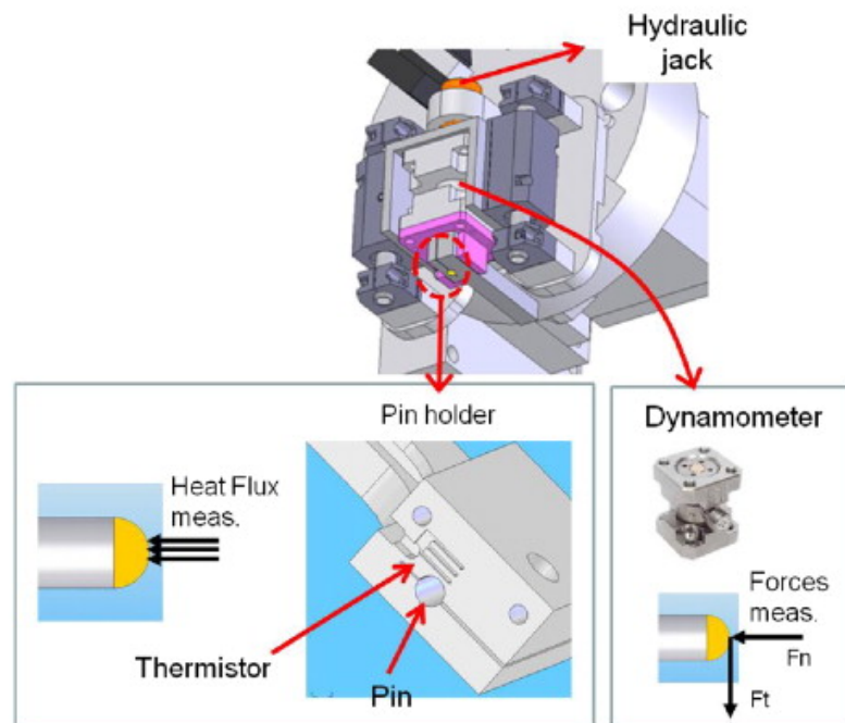
Figure 2.1: Design of the tribometer developed [84].
