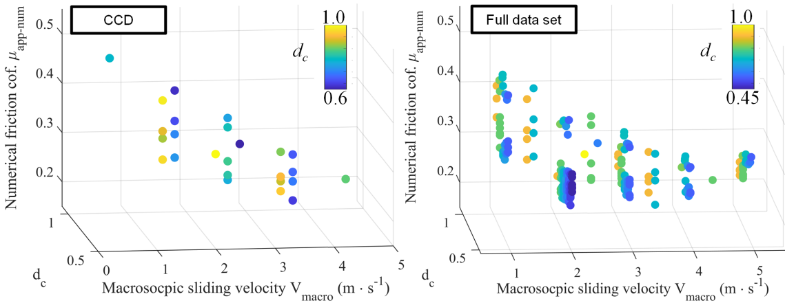
Figure 4.9: Scatter of the numerical apparent friction coefficient ( \mu_{\text{app-num}} ) depended on macroscopic sliding velocity V_{\text{macro}} and decay constant d_c .
