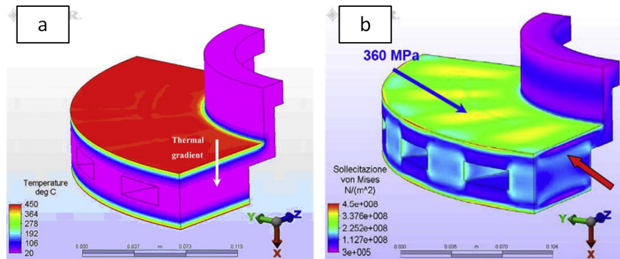
Figure 1.19: Temperature (a) and Von Mises compression stress (b) distribution at the end of braking [64].
