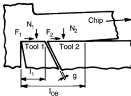
Figure 1.22: Schematic view of the split tool [75].
