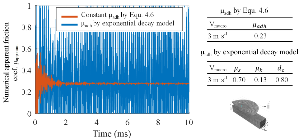
Figure 4.5: Apparent friction coefficient versus time when sliding velocity at 3 m·s -1 .
