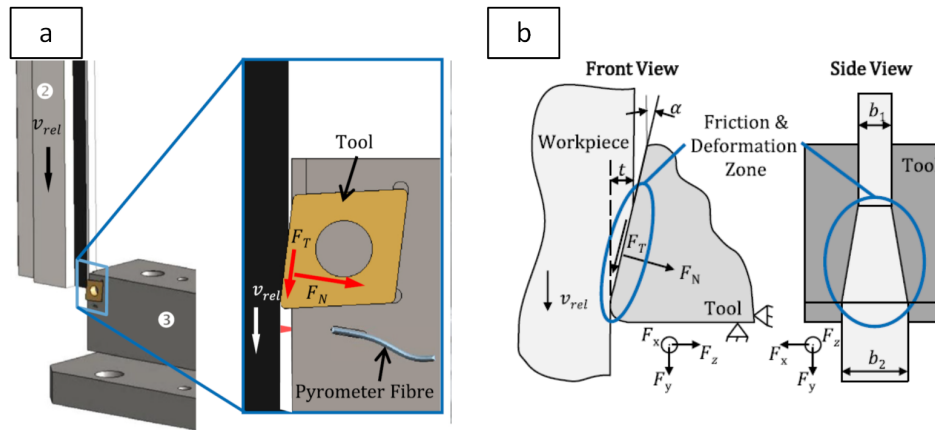
Figure 1.29: Puls' tribometer (a) and kinematic concept (b) [85].
