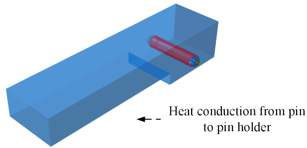
Figure 2.21: Surfaces corresponding the boundary conditions: TCR between pin & pin holder.
