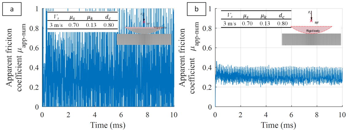
Figure 4.7: Apparent friction coefficient \mu_{\text{app-num}} versus time with a flexible and a fully rigid pin.
