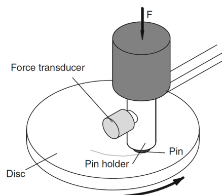
Figure 1.25: Pin-on-disc tribosystem [9].
