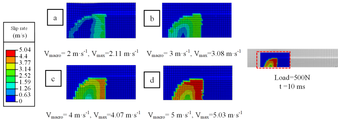
Figure 2.7: Local sliding velocity V_{Is} distribution at the workpiece contact area with different macroscopic sliding velocities V_{macro} V_{macro} (a) 2 m \cdot s^{-1} , (b) 3 m \cdot s^{-1} , (c) 4 m \cdot s^{-1} , and (d) 5 m \cdot s^{-1} .
