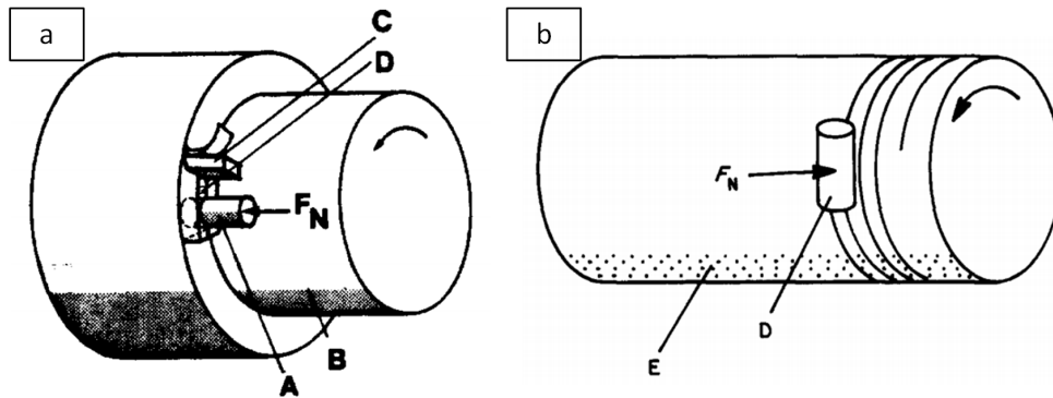
Figure 1.27: Special-designed tribometers:(a) Olsson's tribometer [81], (b) Hedenqvist's tribometer [83].
