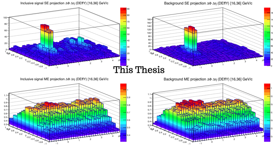
FIGURE 4.32: Top row: Single event distribution in the signal region (left) and sideband region (right). Bottom row: Mixed Event distribution in the signal region (left) and sideband region (right) in the p_T range [16,36] GeV/c.
