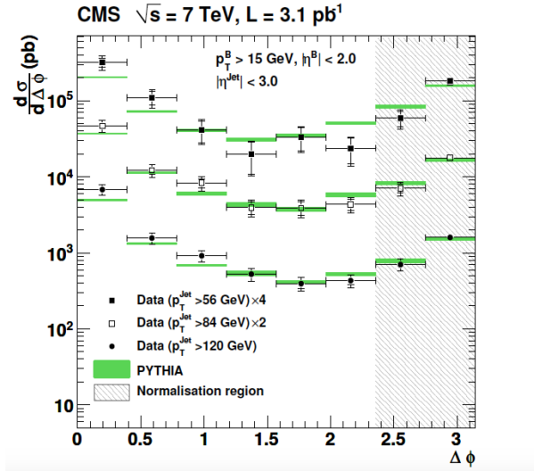
FIGURE 1.40: B\bar{B} differential production cross-section as a function of the opening angle \Delta\phi in p-p collisions at 7 TeV with CMS detector (black filled/empty squares/ black circles) versus PYTHIA simulations (green area) [81].
