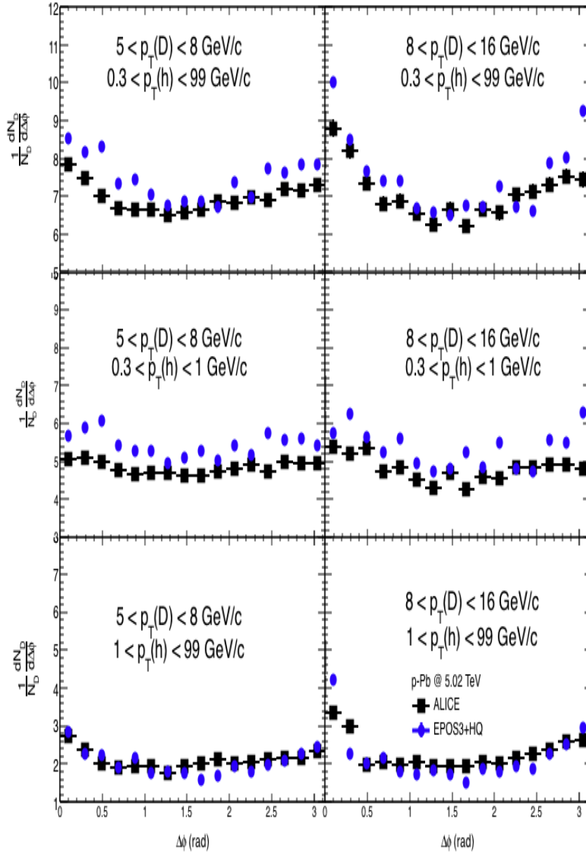
FIGURE 6.24: D-h correlations in p-Pb collisions at \sqrt{s} = 5.02 TeV : ALICE (black squares) vs EPOSHQ (blue circles).
