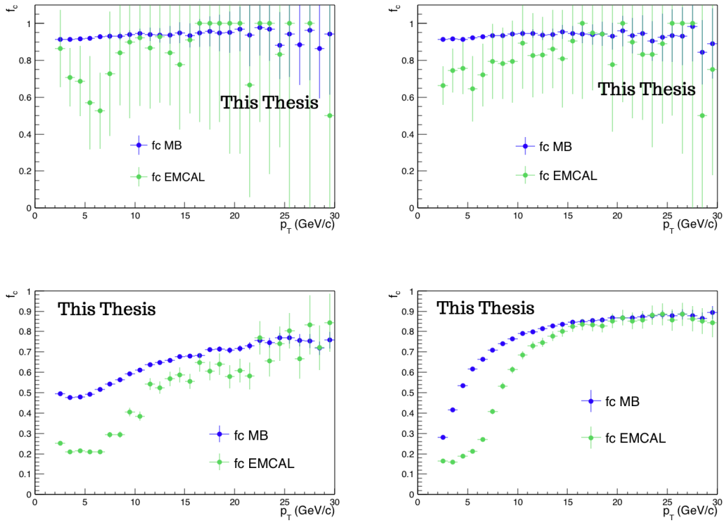
FIGURE 4.41: Fraction of charm quarks as a function of p_T in the case of minimum bias (blue points) and EMCAL trigger (green points) using different MC samples: LHC10f6a (top left), LHC10d4+LHC10f6a (top right), LHC10f7a (bottom left) obtained in pp collisions at 7 TeV and LHC12d2 (bottom right) in pp collisions at 8 TeV.
