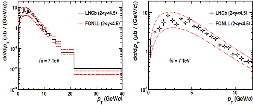
FIGURE 1.13: Left : B^\pm differential production cross section in p-p collisions at 7 TeV with LHCb experiment (black solid line) versus the theoretical prediction from FONLL (red dashed line). Right : Same as the left plot but for a p_T range up to 12 GeV/c [43].
