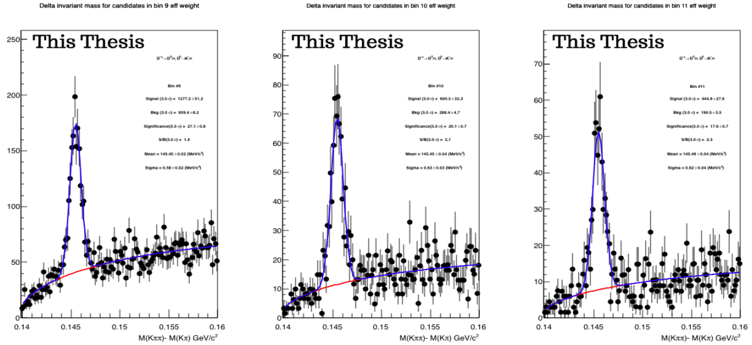
FIGURE 4.5: Invariant mass spectra \Delta M = M(K\pi\pi) - M(K\pi) in the ranges 8 < p_T < 10 \text{GeV}/c (left), 10 < p_T < 12 \text{GeV}/c (middle), 12 < p_T < 16 \text{GeV}/c (right) in minimum bias p-p collisions at \sqrt{s} = 13 \text{TeV} .
