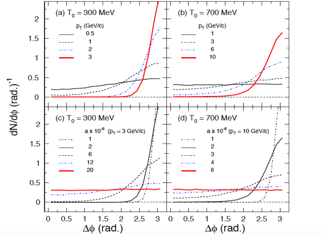
FIGURE 1.33: D\bar{D} correlation distribution as a function of \Delta\phi for the temperature T_0 = 300 MeV (a, c) and T_0 = 700 MeV (b, d) for different initial transverse momentum (top row) and drag coefficients (bottom row) [73].
