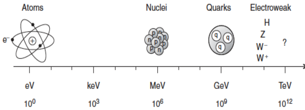
FIGURE 1.3: The components of the matter at different energy scales [4].
