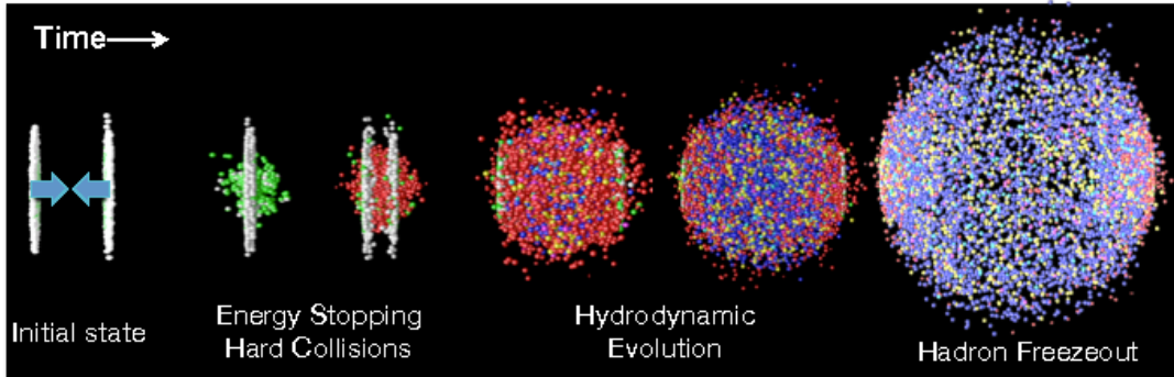
FIGURE 1.9: Spacial-temporal evolution of a central heavy-ion collision.
