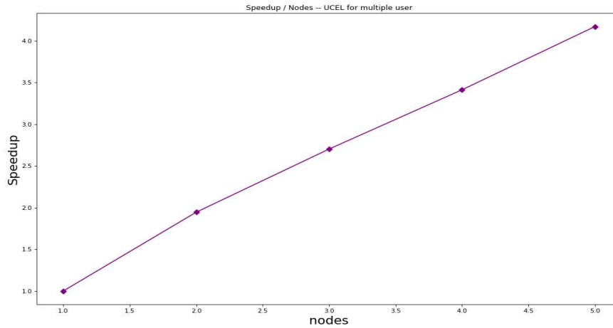
Figure 11.13: UCEL speedup handling 5 users
