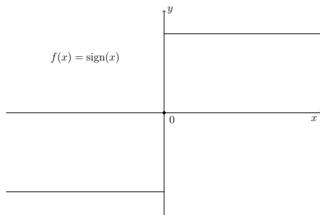
Fig. 2.1: Discontinuous BV function in [-1, 1]
