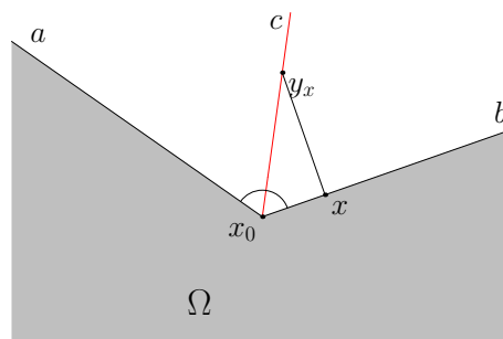
Fig. 2.6: Illustration for Example 2.39
