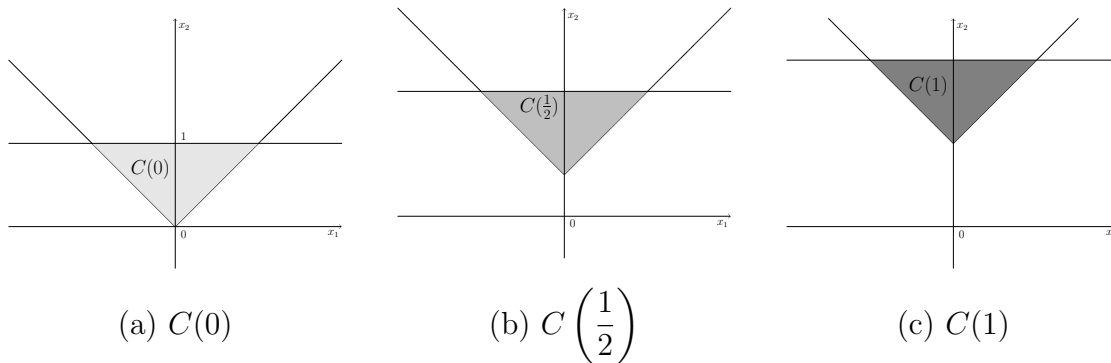
Fig. 3.2: Examples of constraint sets in Example 3.14
