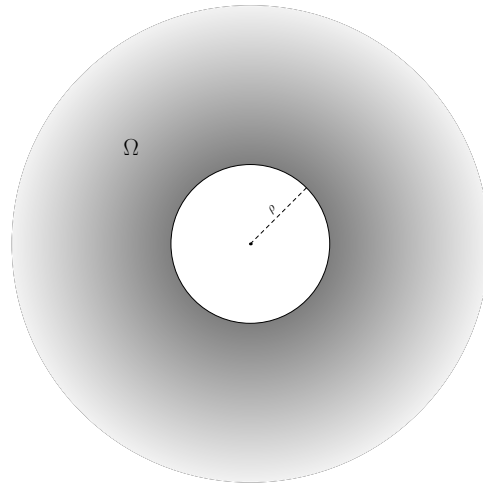
Fig. 2.5: Illustration for Example 2.38 in \mathbb{R}^2
