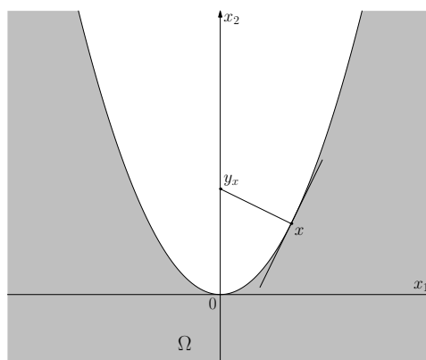
Fig. 4.1: Illustration for Example 4.3
