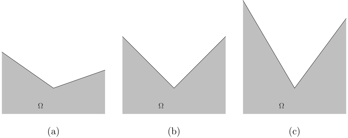
Fig. 2.7: Examples of not uniformly prox-regular sets in \mathbb{R}^2
