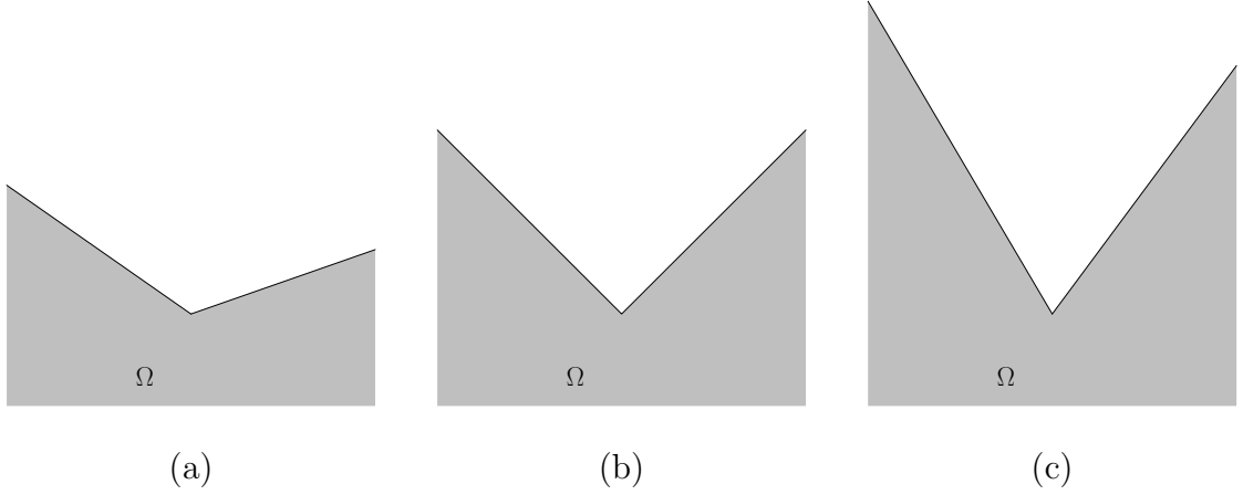
Fig. 2.7: Examples of not uniformly prox-regular sets in \mathbb{R}^2
