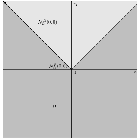
Fig. 2.3: Normal cones of \Omega = \{(x_1, x_2) \in \mathbb{R}^2 \mid x_2 \leq |x_1|\} at (0, 0)
