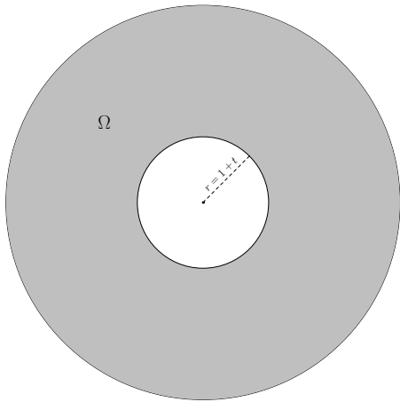
Fig. 4.2: Illustration for Example 4.23
