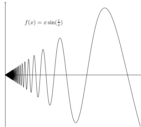
Fig. 2.2: Unbounded variation function in [0, 1]
