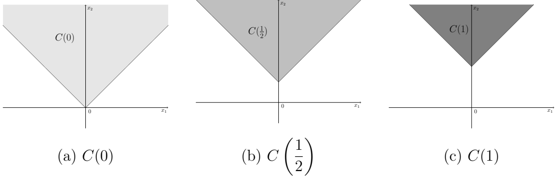
Fig. 3.1: Examples of constraint sets in Example 3.10
