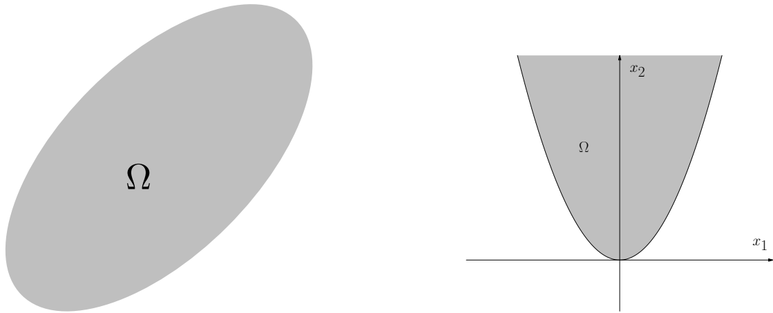
Fig. 2.4: Any convex set is uniformly prox-regular
