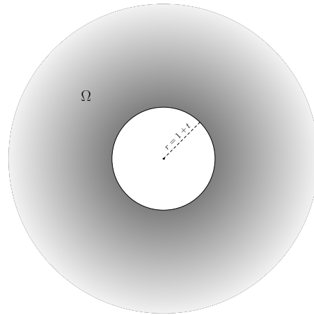
Fig. 4.3: Illustration for Example 4.24
