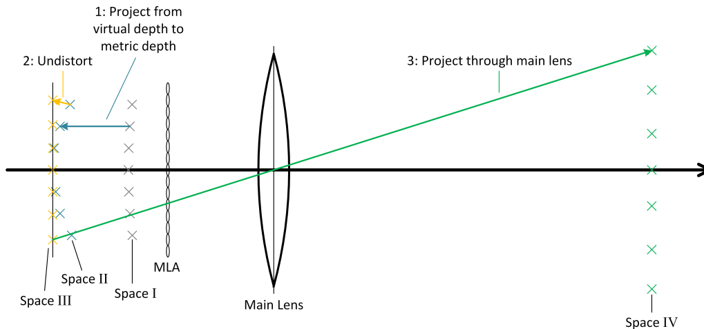
Figure 3.8: Heinze et al. [125] camera model. Virtual point is estimated, then reprojected into metric. Distortion is handled, and the point is projected through the main lens in object space.
