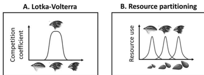
Figure I. 3 Schematic representation of Lotka-Volterra competition. Image from D'Andrea et al., 2019
