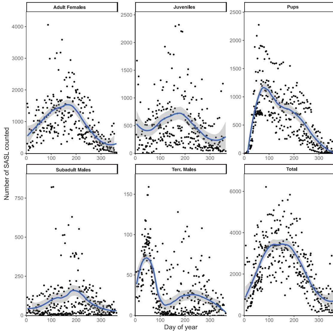
Figure A. 2 Multi-panel plot of South American sea lions counts by age-class according to day of year collected at the main breeding site N7 in Punta San Juan, Peru. Classes include: Adult Females, Juveniles, Pups, Subadult Males and Territorial Males. Total is the sum of all the age-classes. Blue line is a fitted loess model to depict the trend in abundance throughout the year. Data points include all study years available for site.
