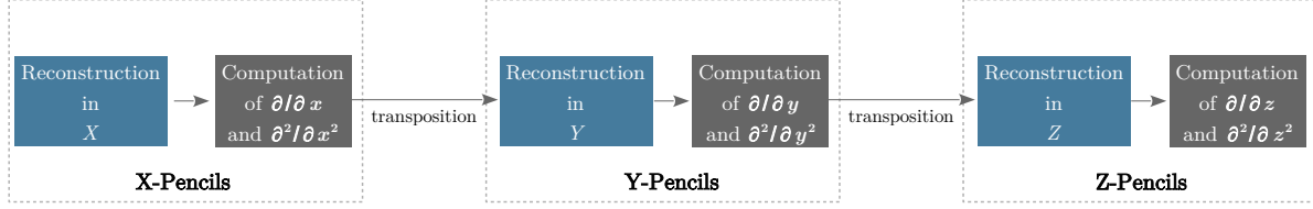
Figure 2.5: Schematic diagram of the 1D interpolations in the framework of the 2D decomposition implemented in Incompact3d.
