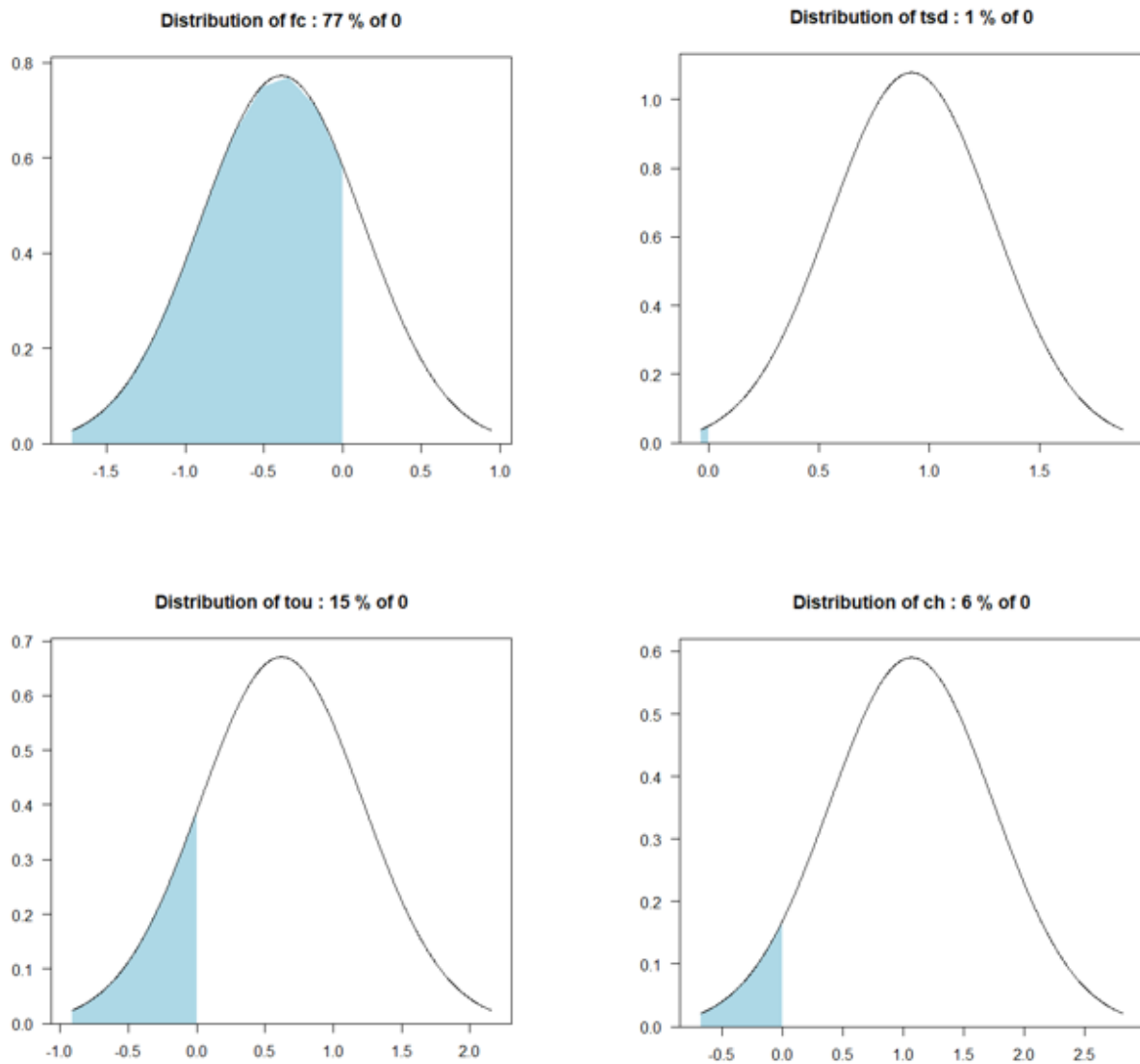
Figure 3.10. – Distribution of random parameters of individuals for the final MXL model of the Cévennes sample.
