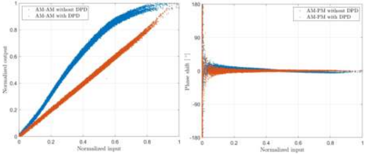
(a) AM-AM without and with DPD
