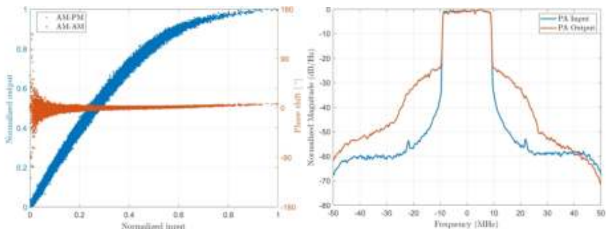
(a) AM-AM and AM-PM curves
