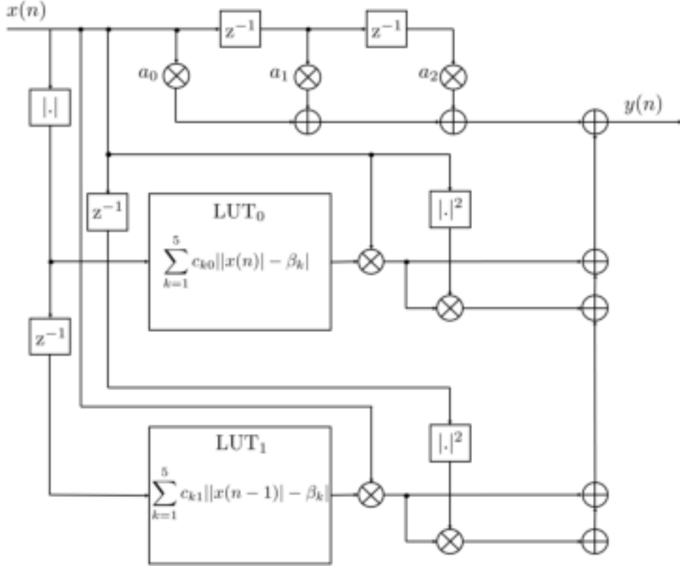
Figure 4.10: Implementation of optimal DVR model by LUT
