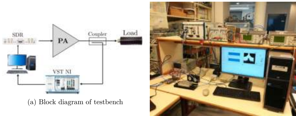
(b) Testbench of LDMOS PA
