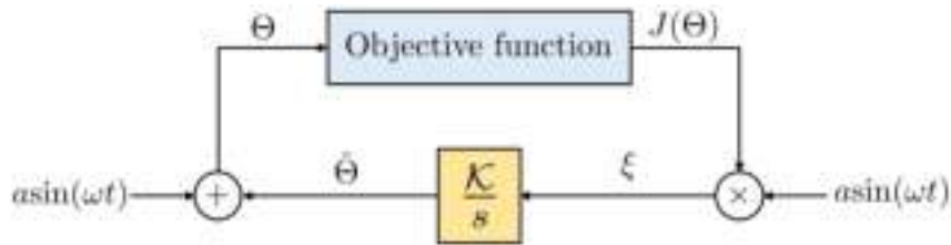
Figure 5.10: ESC scheme
