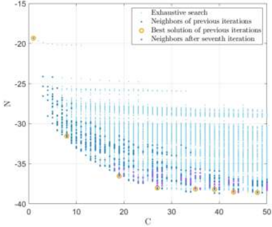
Figure 3.32: Evolution of HC algorithm after seventh iteration
