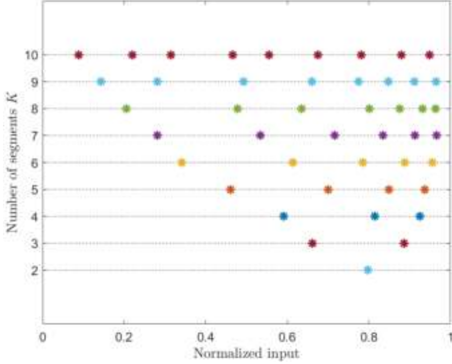
Figure 3.21: Optimal segmentation versus number of segments K
