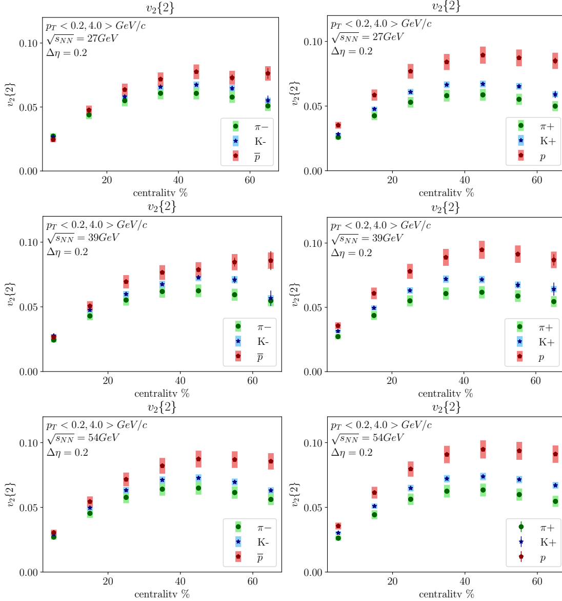
Figure 5.7 – 2PC integrated over p_T v_2\{2\} for Au+Au collisions at \sqrt{s_{NN}} = 27, 39 and 54.4 \text{ GeV} in function of centrality. The \Delta\eta = 0.2 and the p_T range is 0.2 to 4.0 \text{ GeV}/c . This thesis
