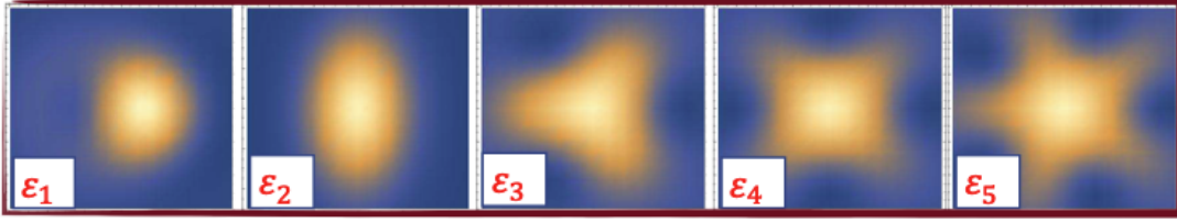
Figure 2.6 – Eccentricities \varepsilon_n with the corresponding participant zone shape [54].
