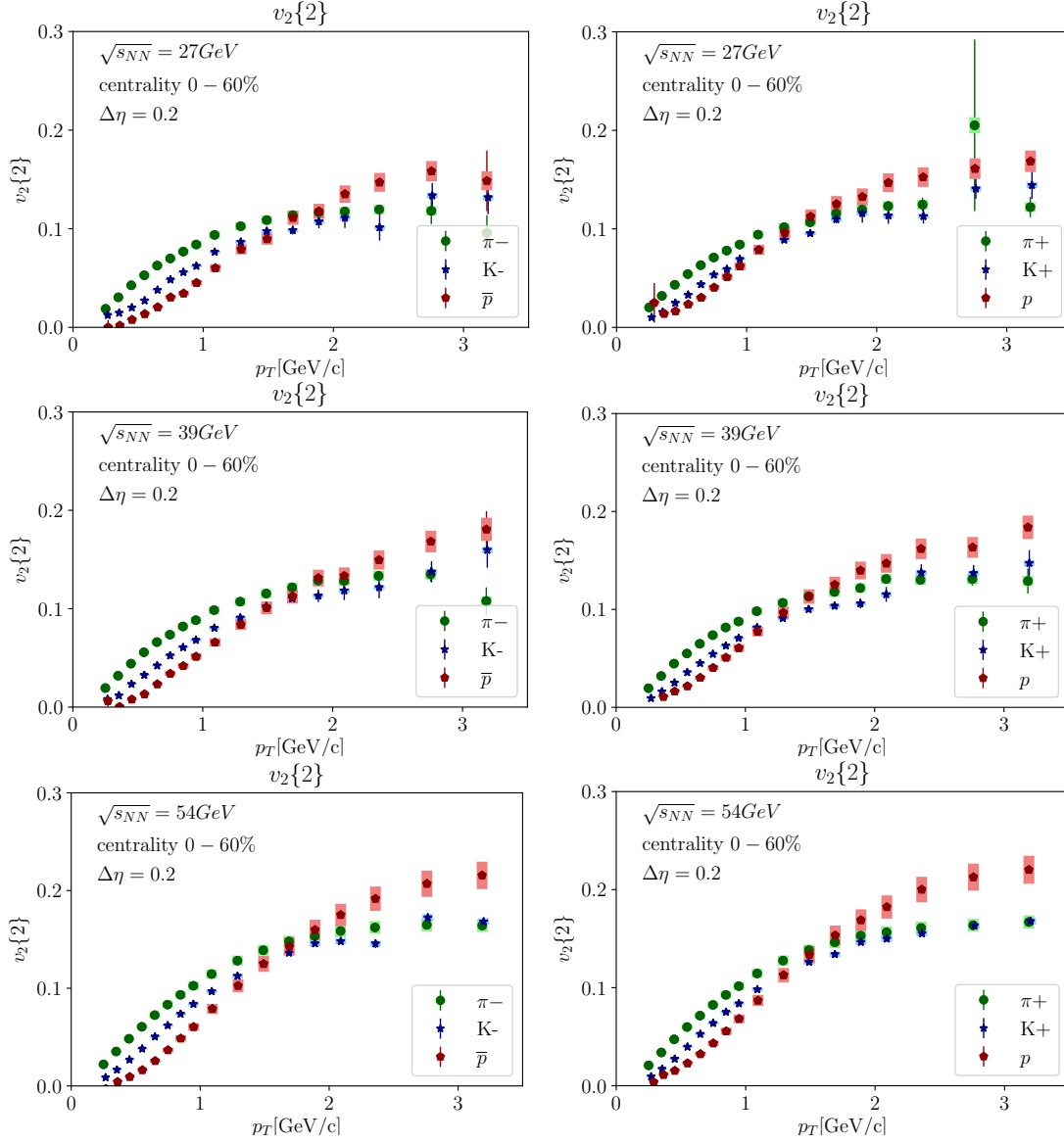
Figure 5.11 – 2PC p_T -differential v_2\{2\} for Au+Au collisions at \sqrt{s_{NN}} = 27, 39 and 54.4 GeV in centrality 0 - 60\% . The \Delta\eta = 0.2 . This thesis
