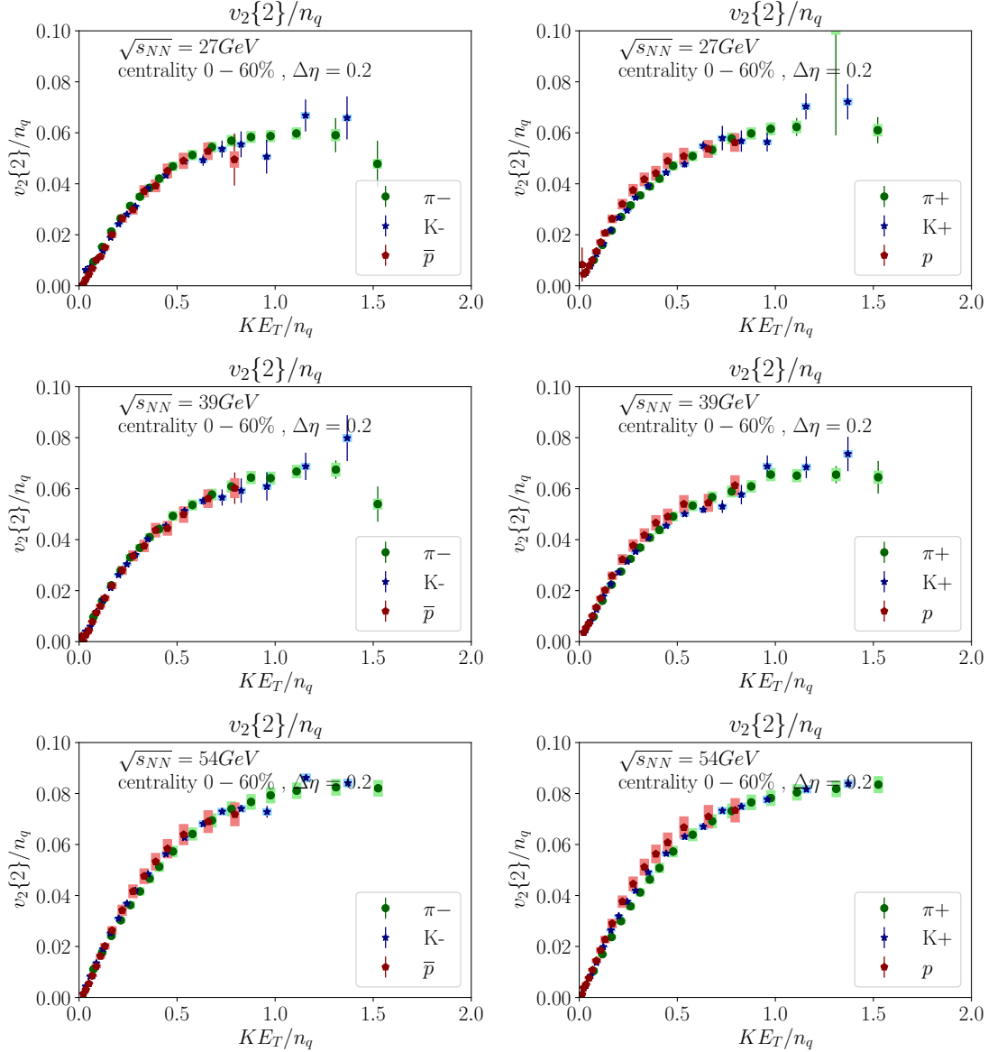
Figure 5.13 – 2PC p_T -differential v_2\{2\} for Au+Au collisions at \sqrt{s_{NN}} = 27, 39 and 54.4 GeV in centrality 0 - 60\% scaled with number of constituent quarks ( v_n\{2\}/n_q^{n/2} ) in function of transverse kinetic energy KE_T . This thesis
