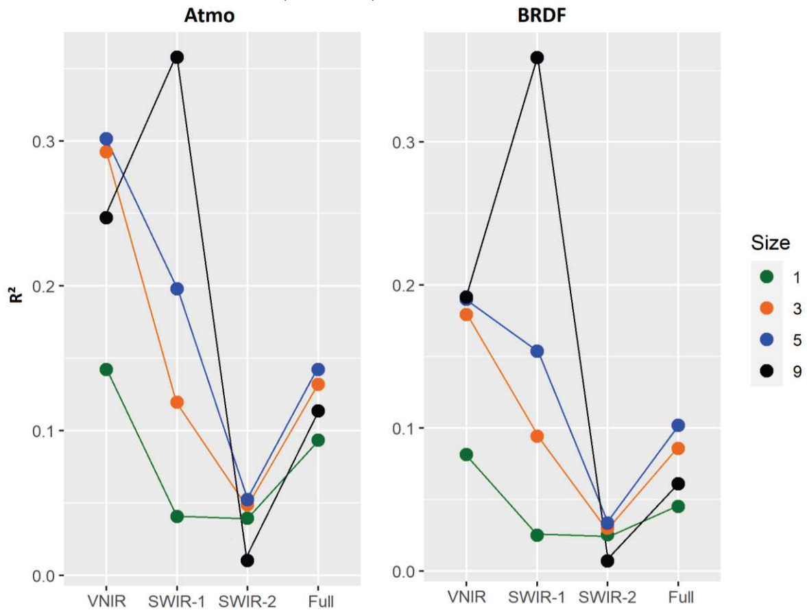
Figure 14: Comparison of variance explained using atmospheric correction data prior (left) or after (right) applying BRDF correction. Permissive illumination was used in both cases.
