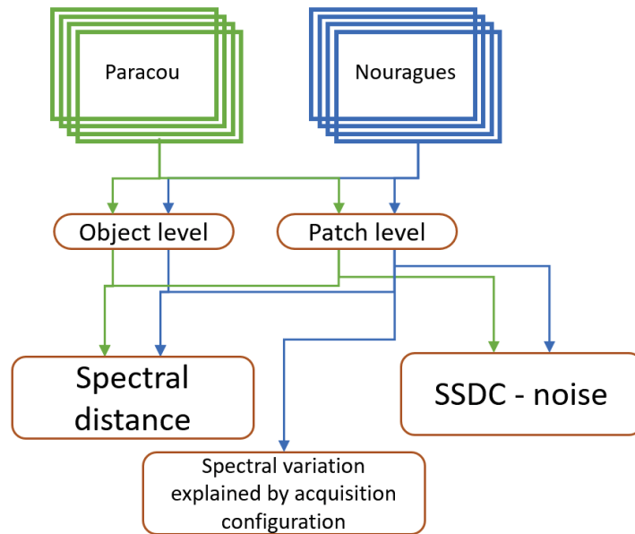
Figure 1: Workflow of the study. The blue boxes refer to hyperspectral imageries. The oranges boxes refer to the methods used in the study.
