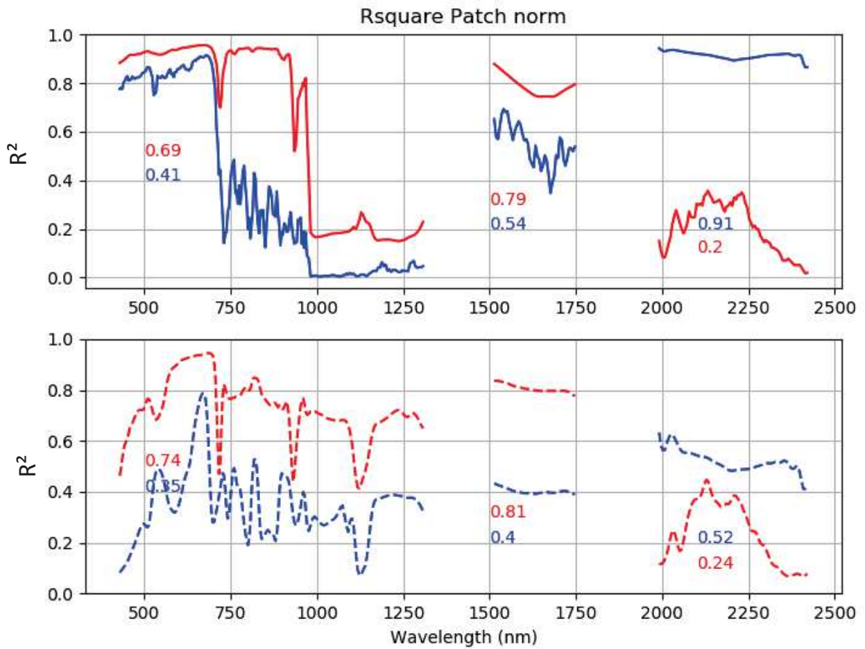
Figure 8: Relation between same patch (5x5 pixels) viewed at the two dates in Paracou (full lines) and Nouragues (dashed lines) site. The blue and red lines represent the dataset no corrected and corrected by atmospheric correction respectively.
