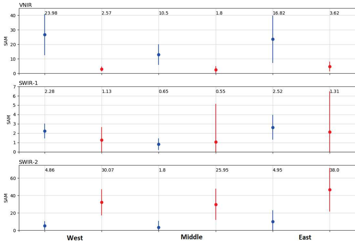
Figure 10: Characterization of spectral dissimilarity by the SAM index (5x5 patches) at the Nouragues site in three sub-zones (left to right) and three spectral ranges (top to bottom). Blue and red symbols stand for radiance and reflectance data respectively.
